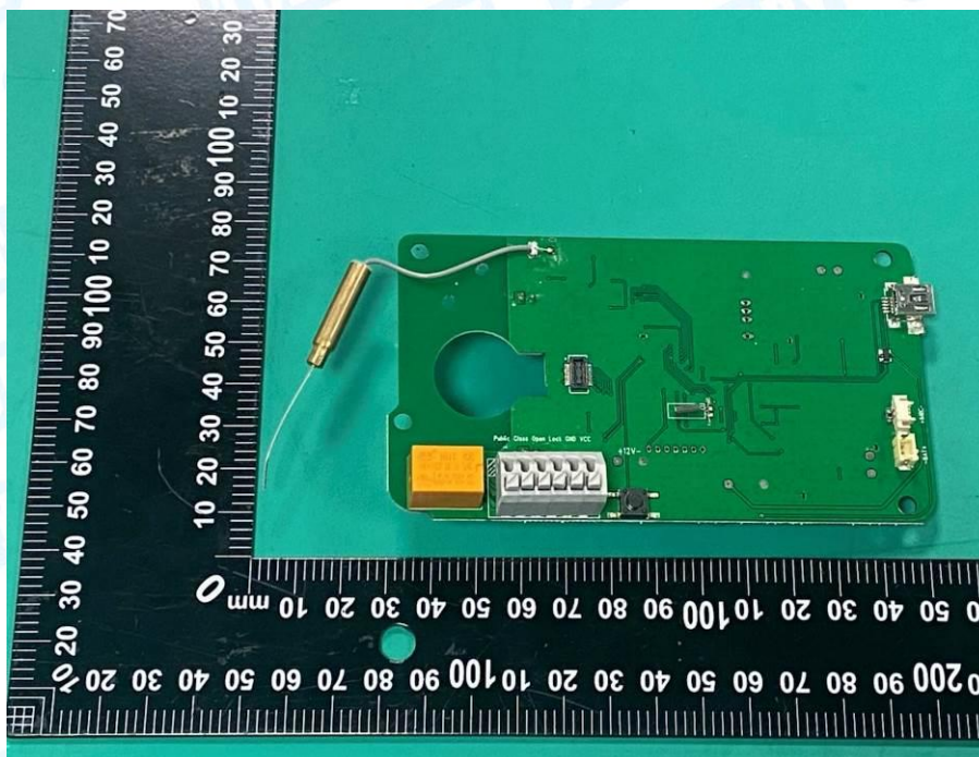
Photo 19 Appearance of PCB
