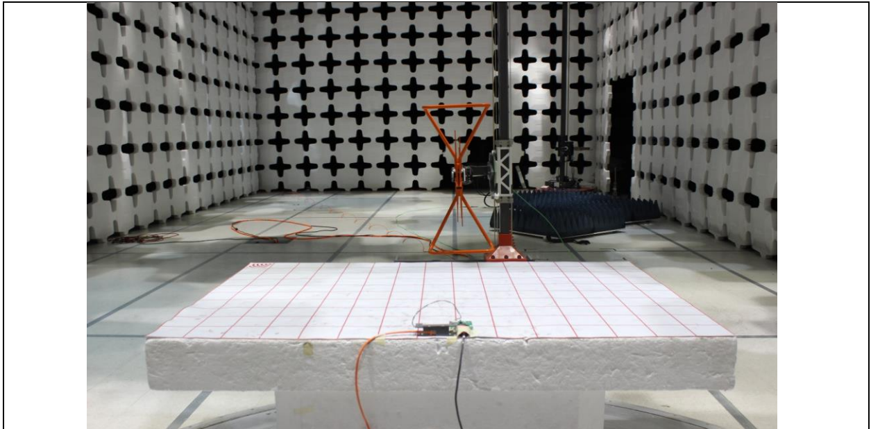
Radiated Emission Test Below 1GHz Front View
