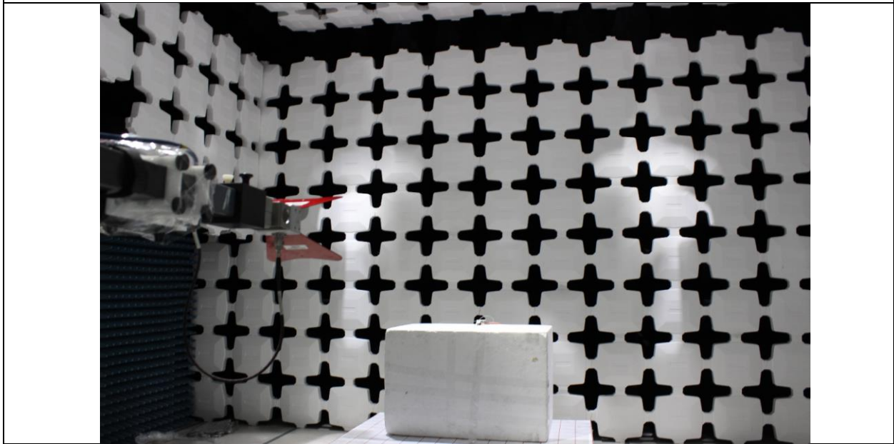
Radiated Emission Test Above 1GHz Rear View
