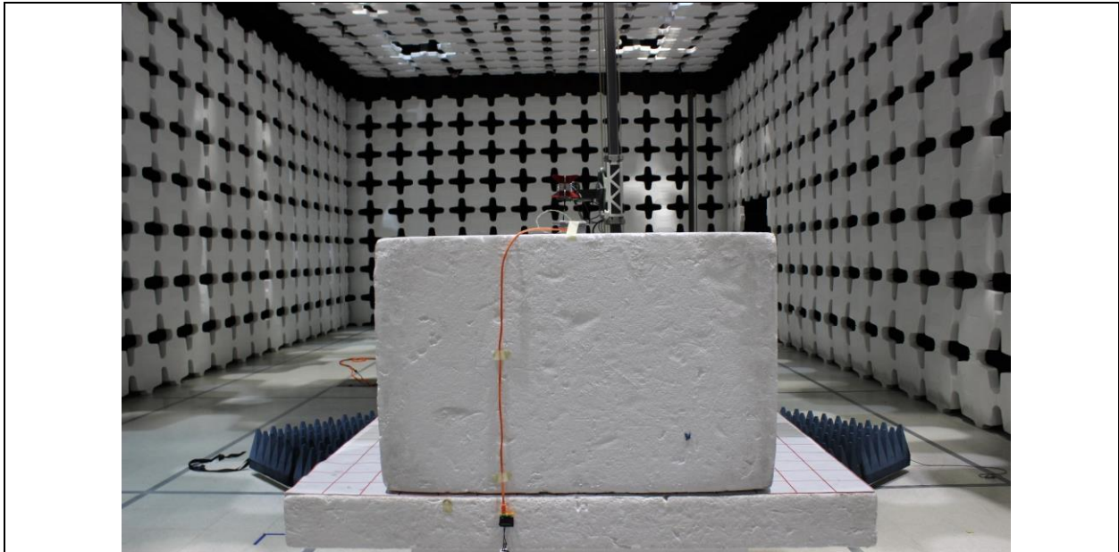
Radiated Emission Test Above 1GHz Front View
