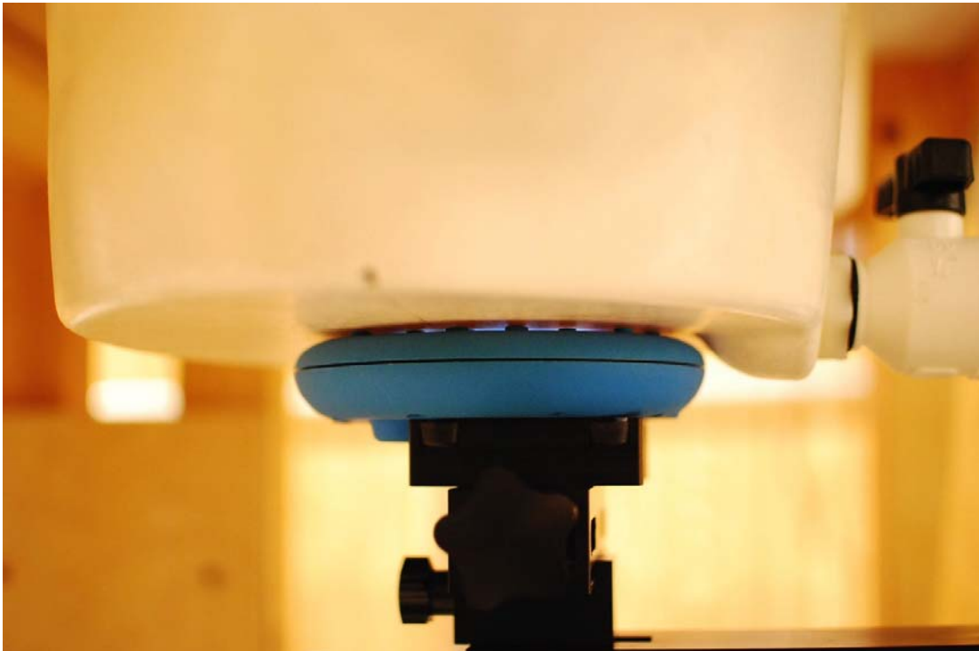
Figure 18-8 SAR Test Setup Photo 8: Front Side
