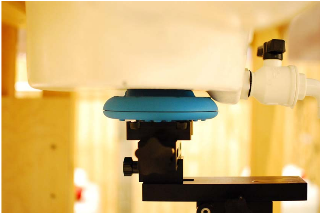
Figure 18-4 SAR Test Setup Photo 4: Back Side
