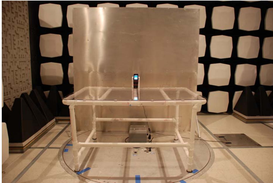
Worst-case conducted emission, front view
