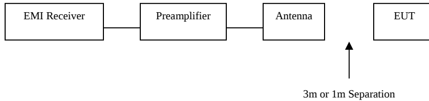
MP-FS-RX2, Radiated Spurious Emissions
