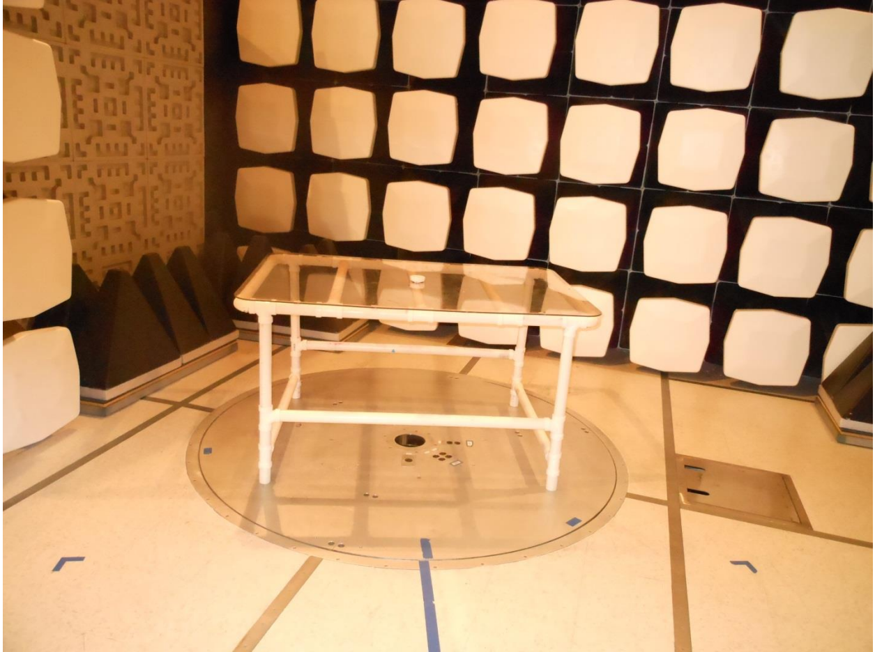
EUT ceiling mount position
