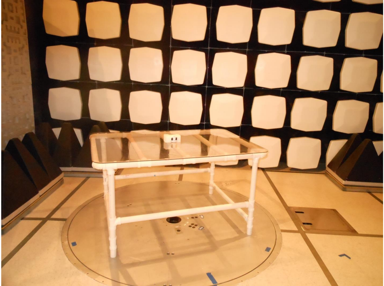
EUT wall mount position
