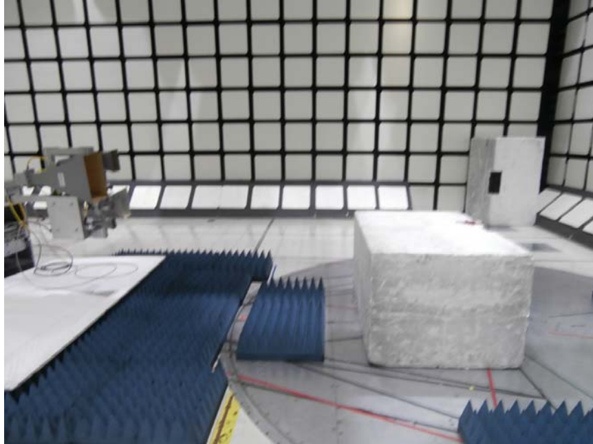
Worst-case radiated emission, Side view
