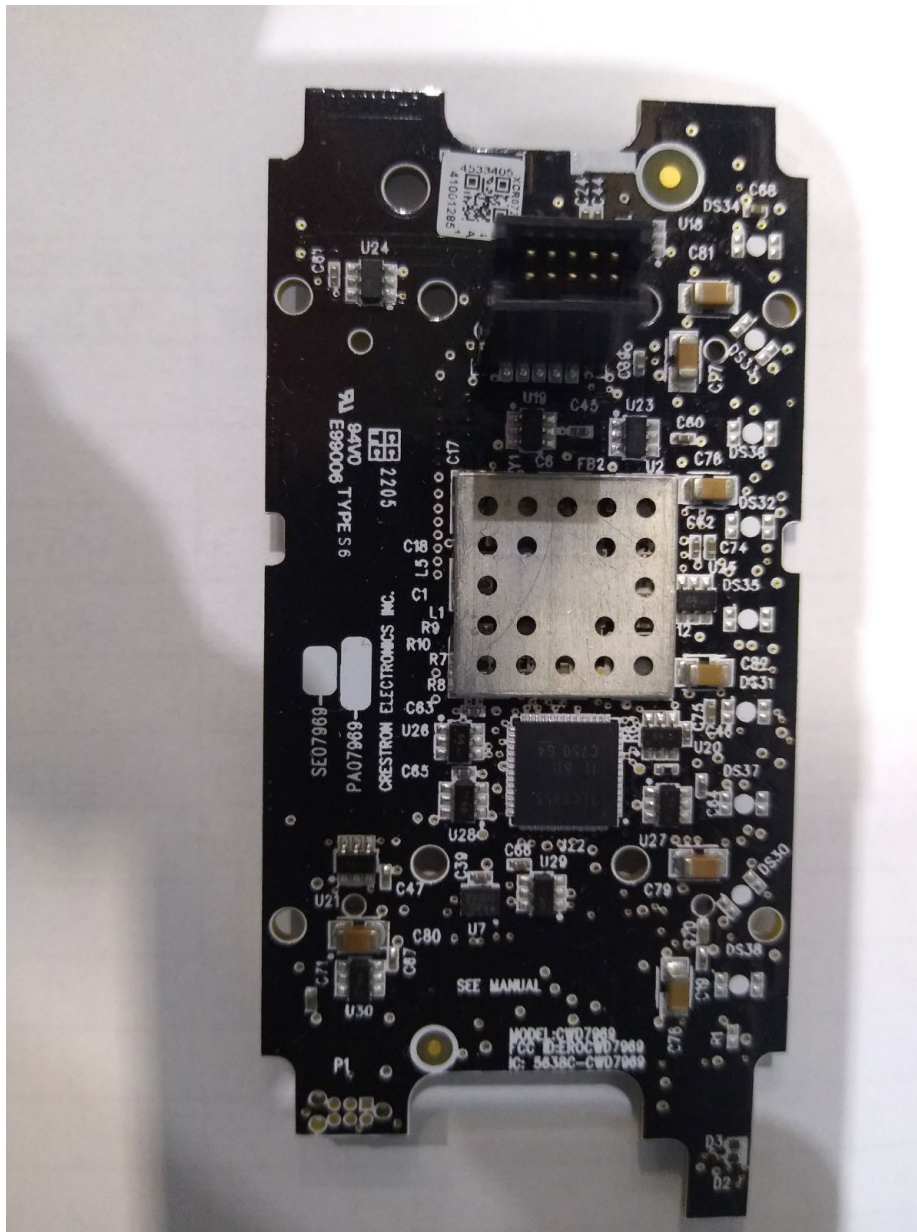
Internal Photo of bottom of radio board with the shield
