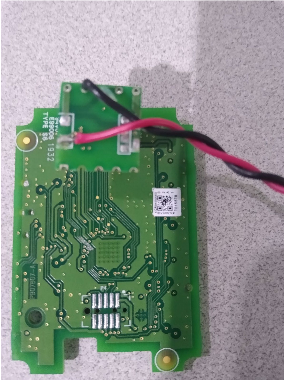
REAR VIEW WITH POWER ADAPTER BOARD CONNECTED
