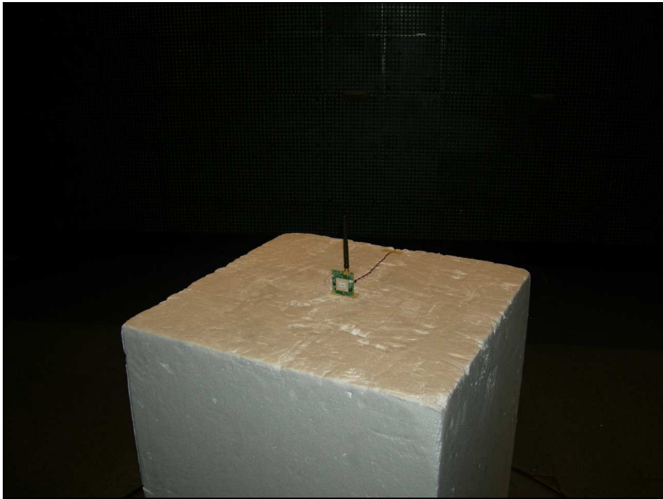
Figure 7: Radiated Emissions – Dipole Antenna – YPOS
