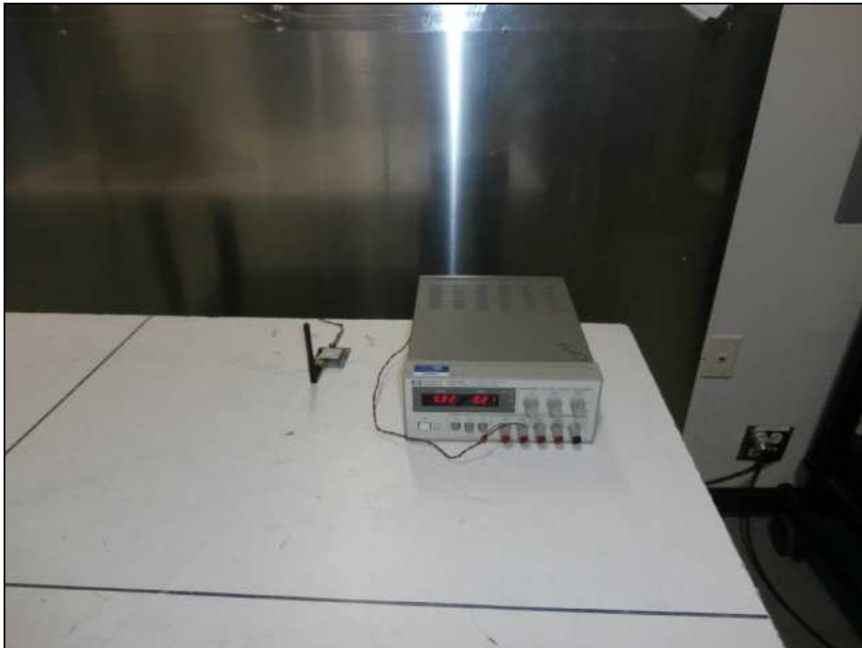
Figure 11: Conducted Emissions – Front View – Dipole Antenna
