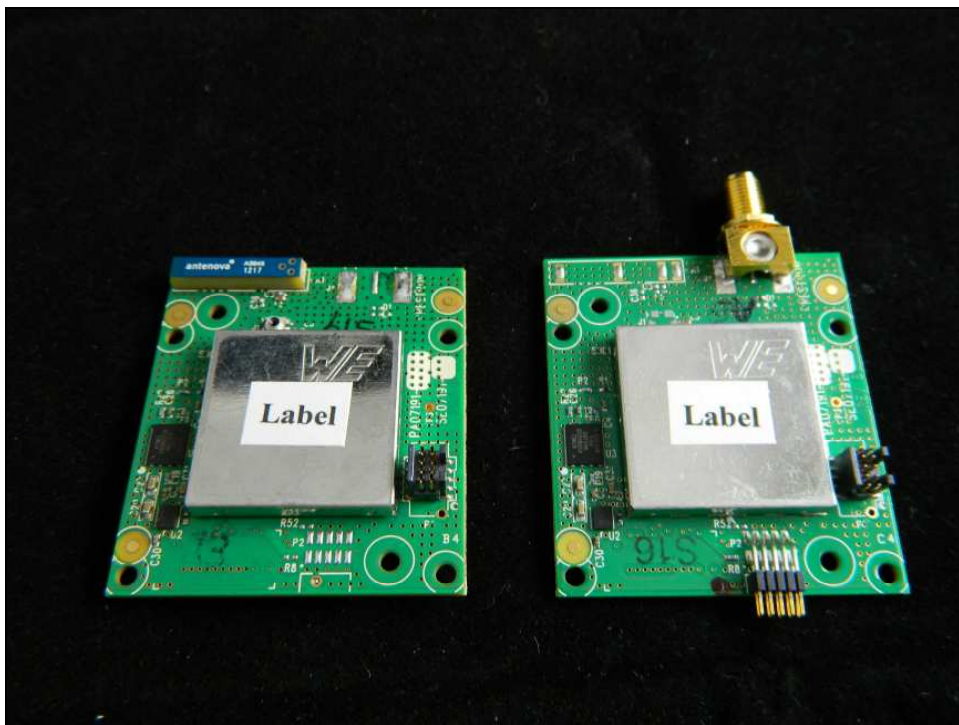
Figure 1: Label Placement
