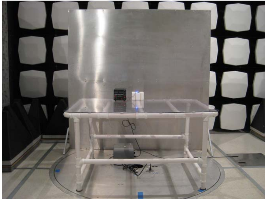
Worst-case conducted emission, front view
