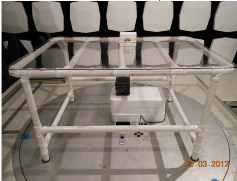
Worst-case radiated emission, front view
