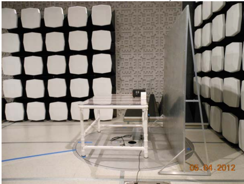
Worst-case conducted emission, side view
