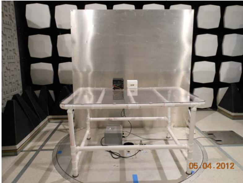
Worst-case conducted emission, front view
