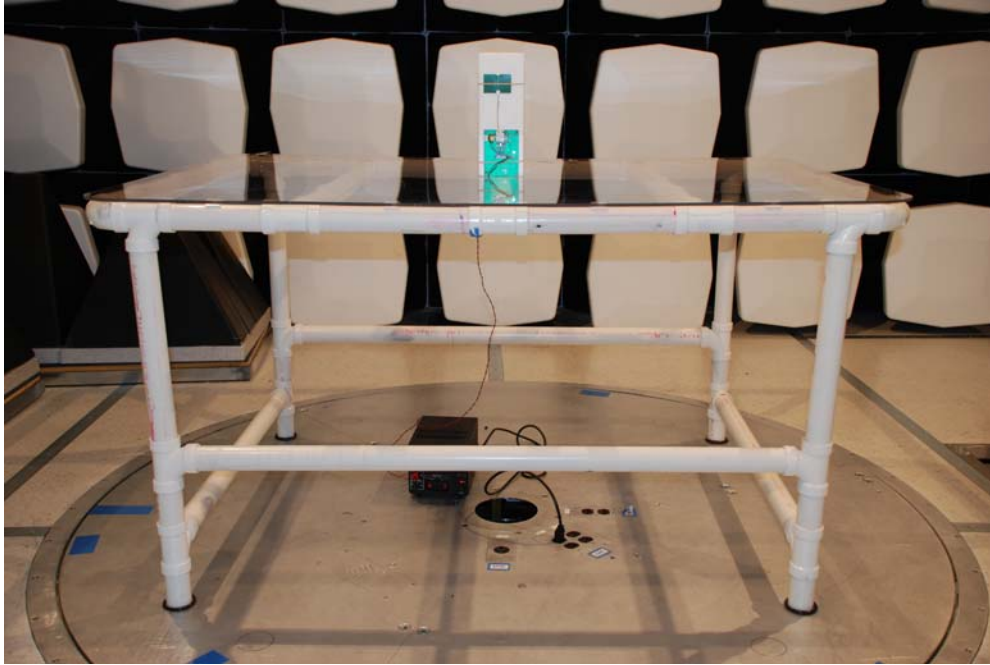
Worst-case radiated emission, front view
