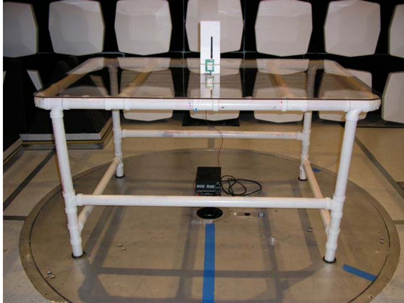
Worst-case radiated emission, front view
