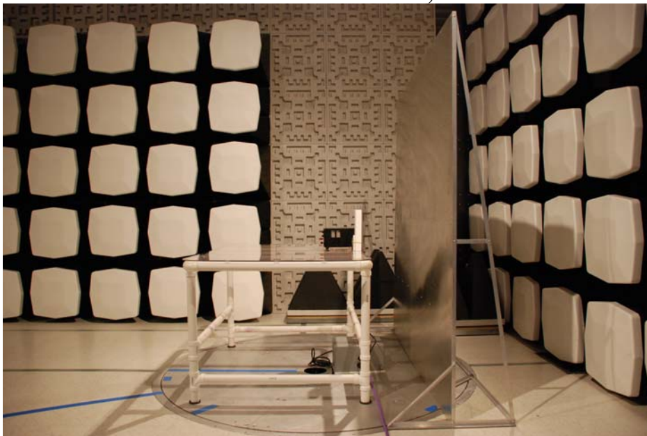
Worst-case conducted emission, side view
