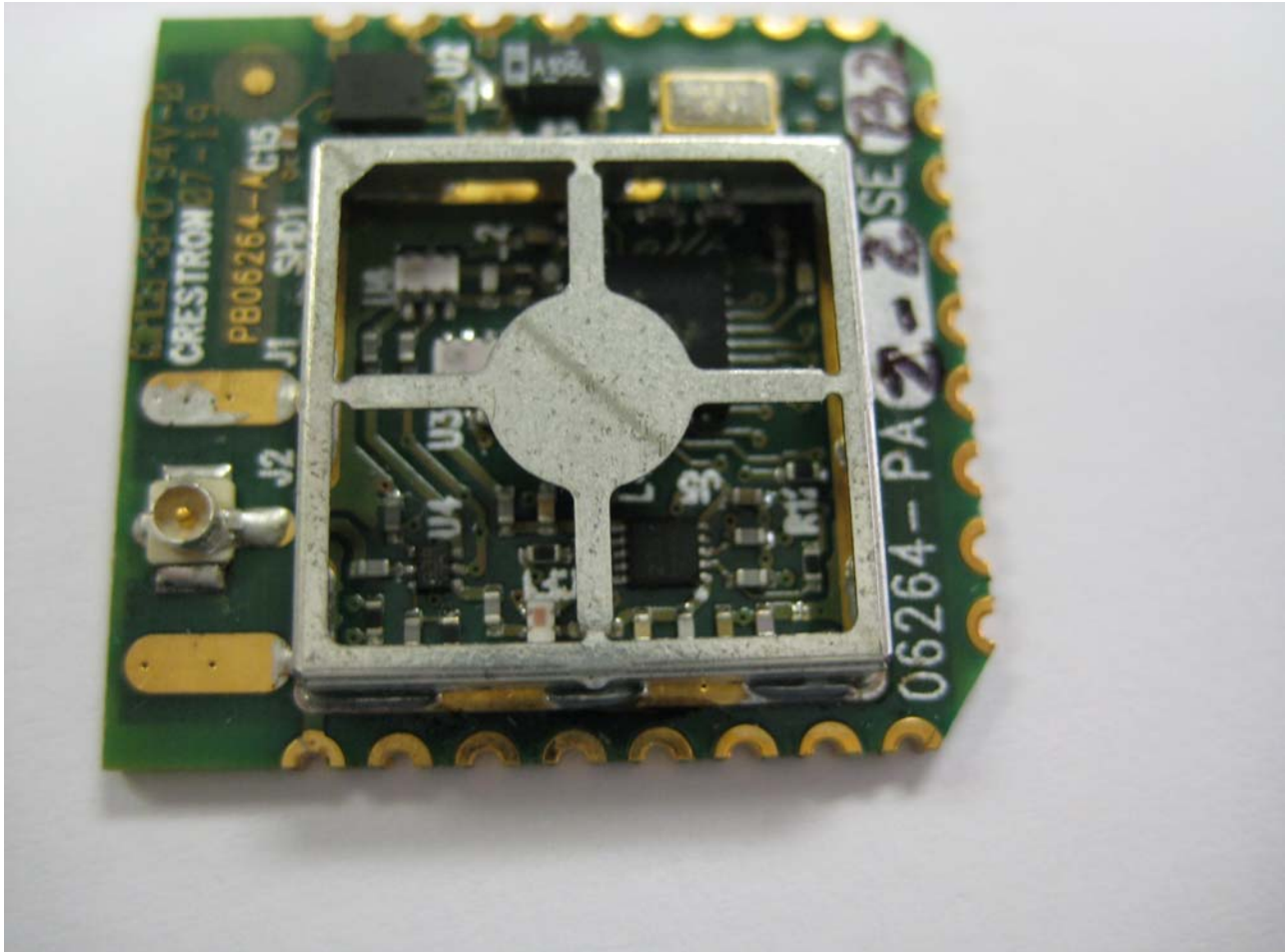
View #3 of RF Section, Shield Removed
