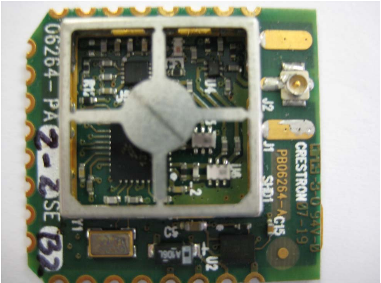
View #5 of RF Section, Shield Removed
