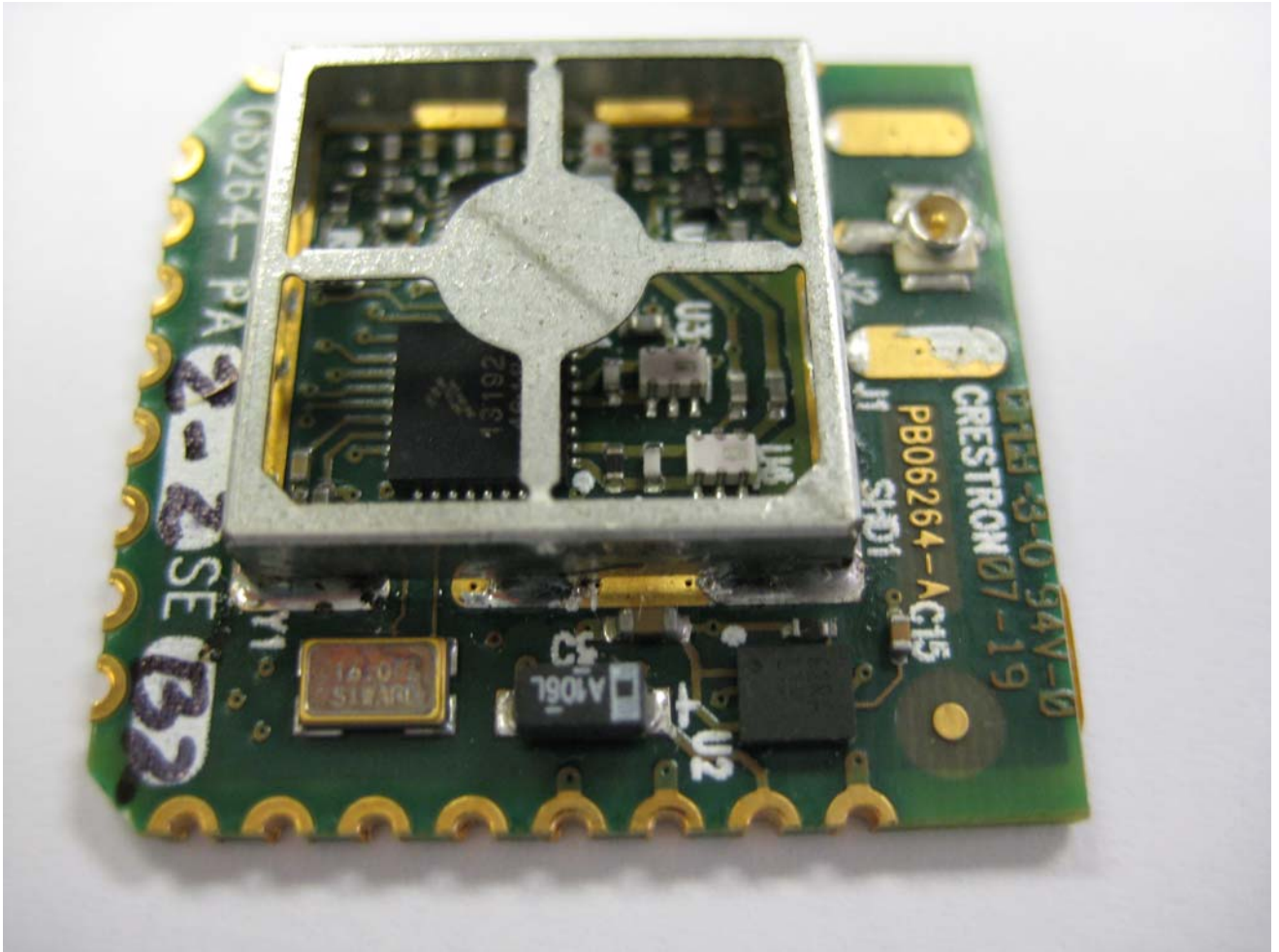
View #4 of RF Section, Shield Removed
