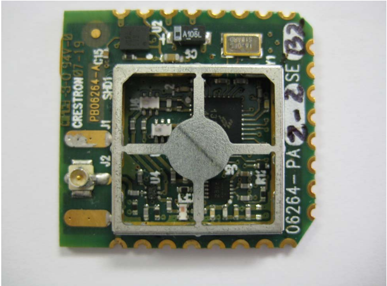
View #2 of RF Section, Shield Removed
