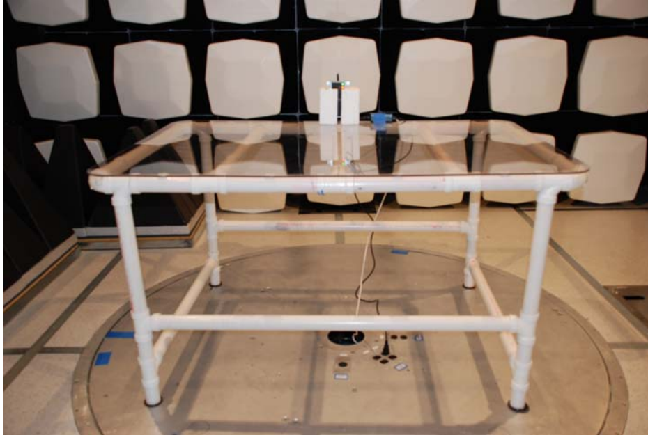
Worst-case radiated emission, front view, LAN PoE port
