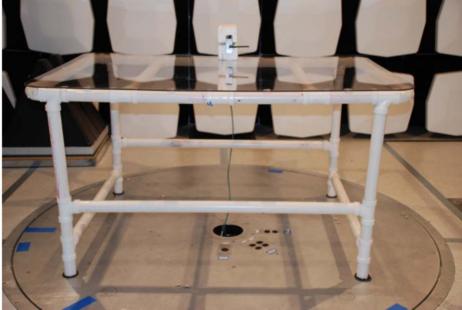
Worst-case radiated emission, front view, Cresnet port
