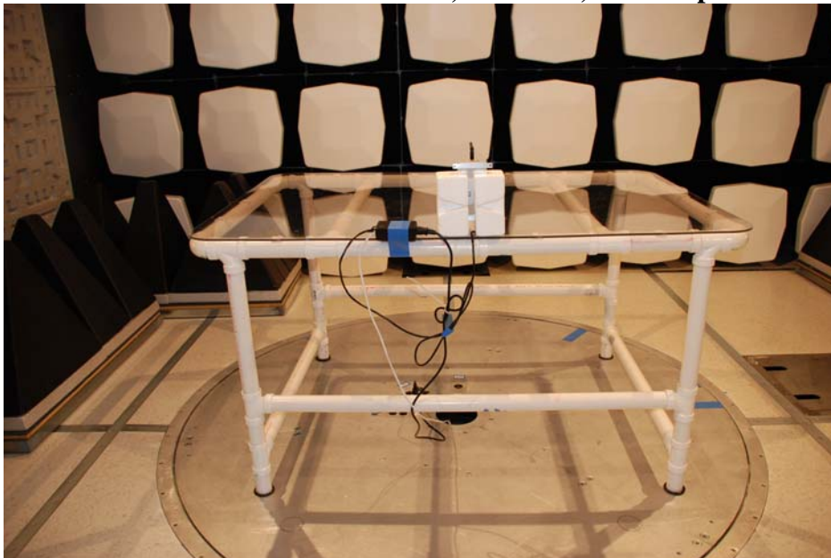
Worst-case radiated emission, rear view, Cresnet port
