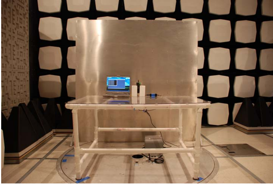
Worst-case conducted emission, front view, LAN PoE port
