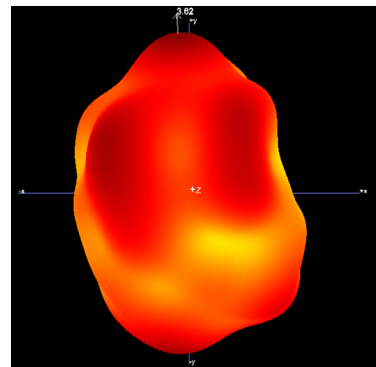
5G 3D
