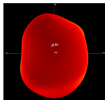
2.4G phi=90deg
