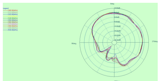
2.4G phi=90deg
