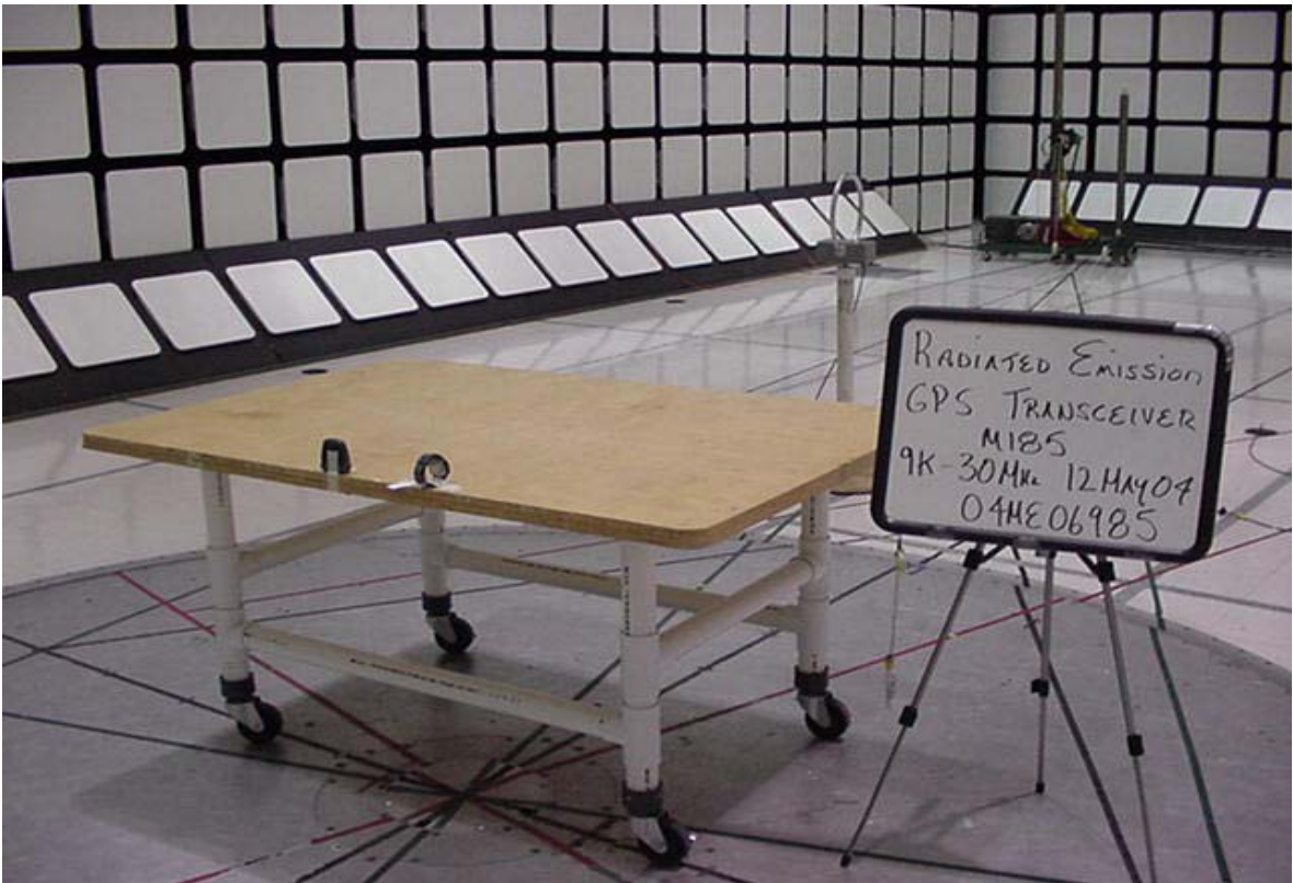
Radiated Emissions Rear – 9kHz-30MHz
