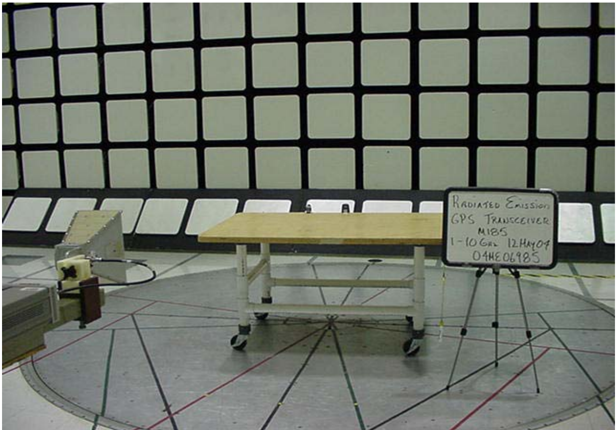
Radiated Emissions Front – 1-10GHz
