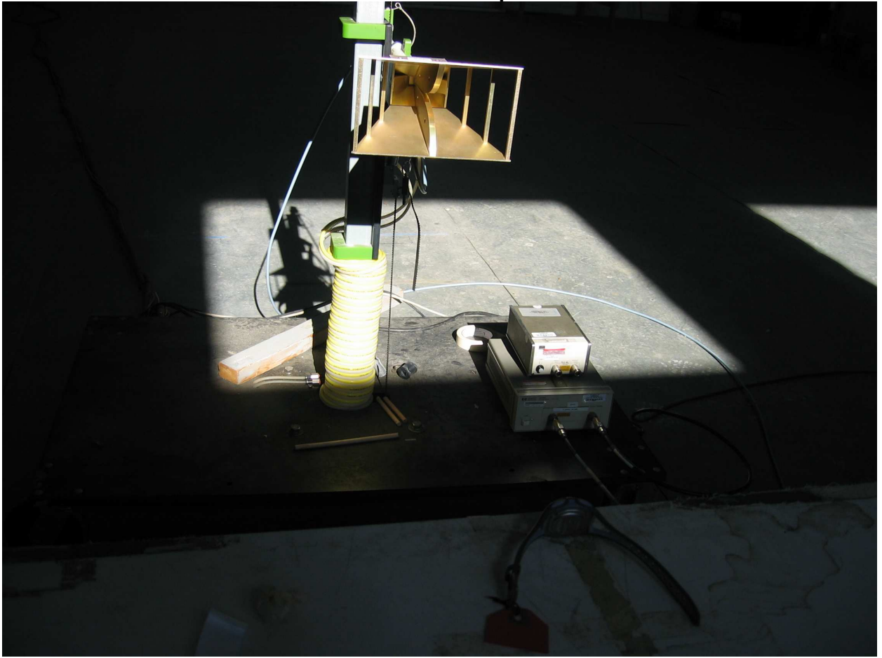
Rx Radiated Emissions Setup Photo 2
