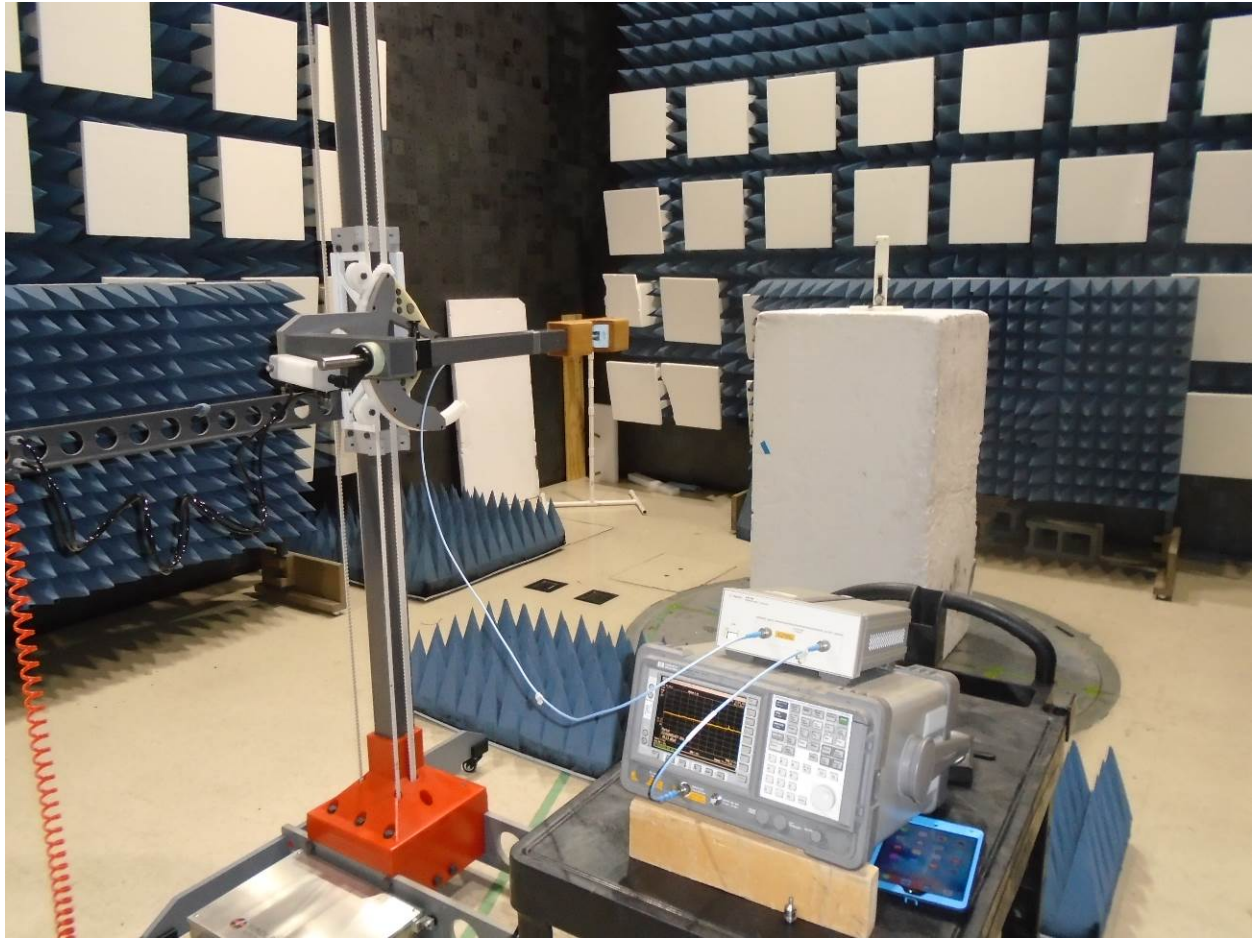
Figure 4: Typical Radiated Emissions – 18 GHz to 25 GHz shown, Front view
