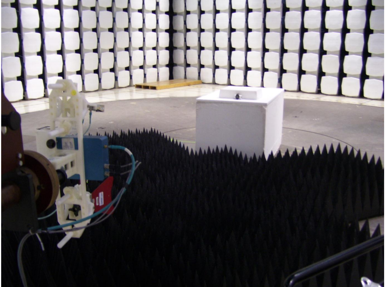
Figure 1: Test Setup Photo View- Field Strength and Radiated Emissions
