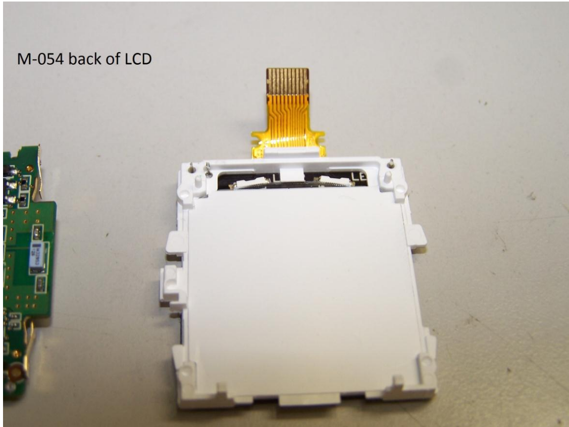
Figure 7: Internal View – Back of LCD
