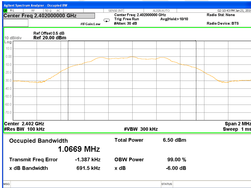
6dB Bandwidth TX CH00
