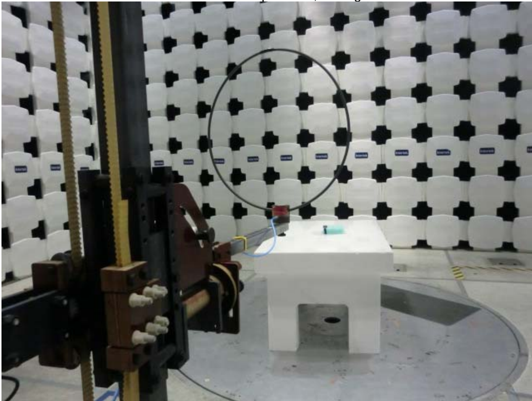
Fundamental Test Setup Photos, Orthogonal # 1
