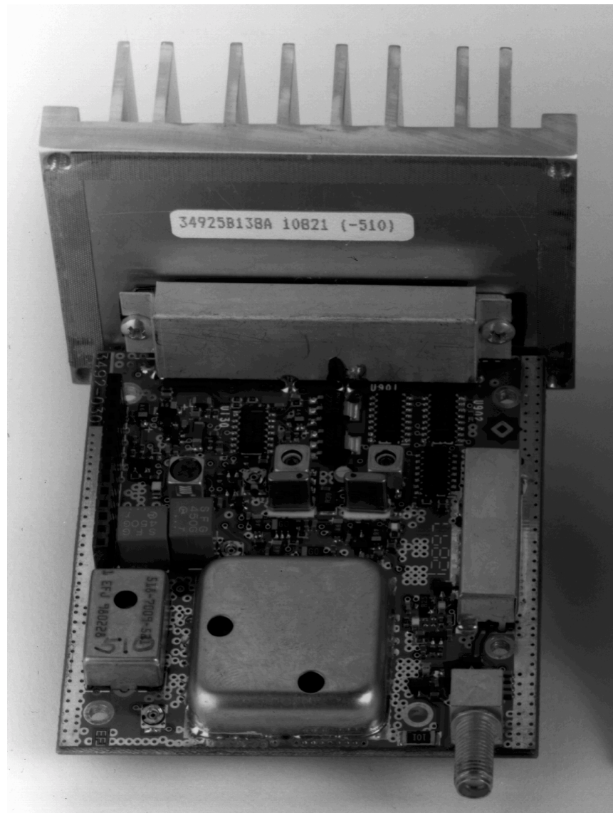
Fig2. MCUC5 –transceiver board, bottom ( to loader/modem board) side view
