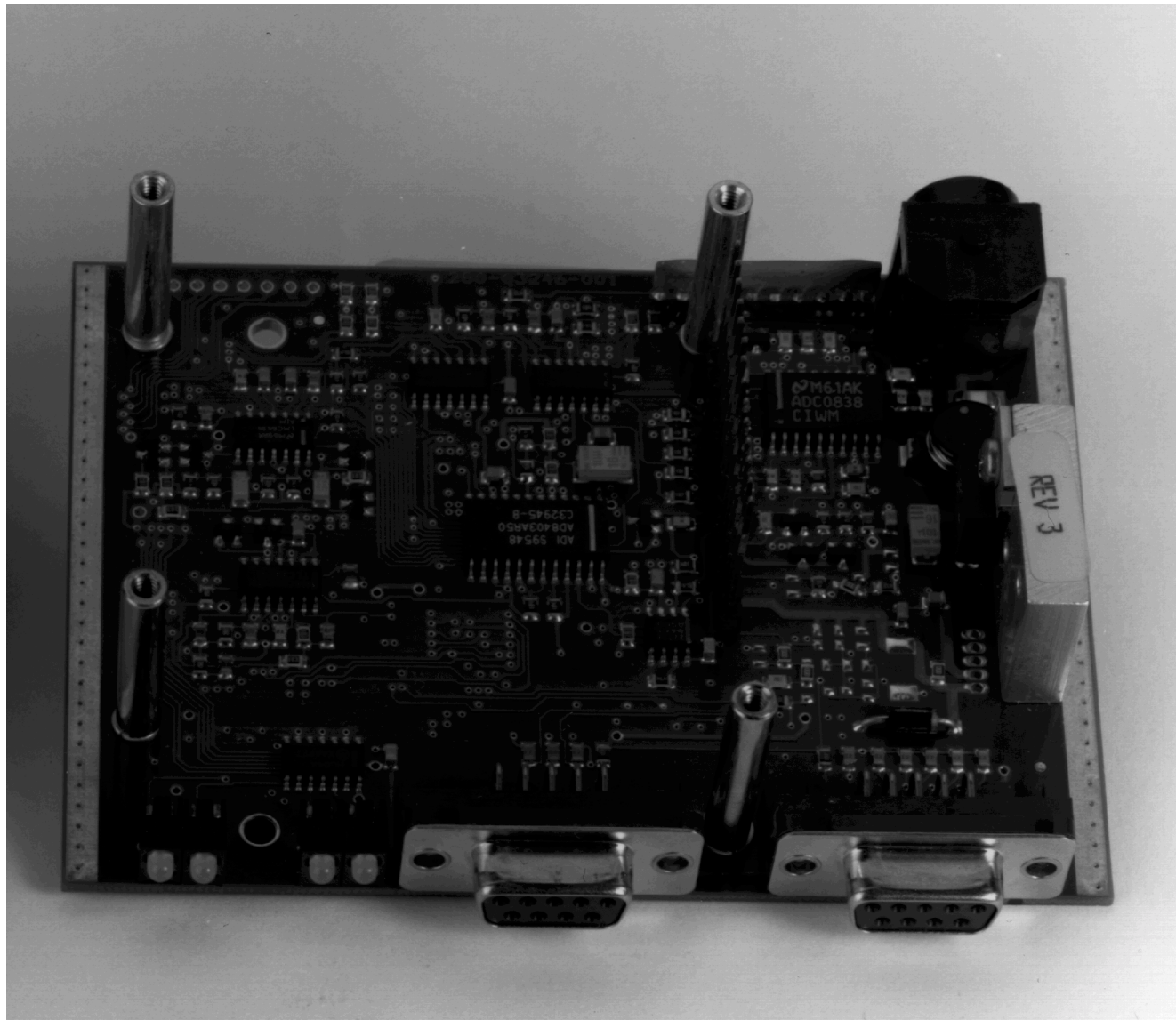
Fig4. MCUC5 -loader/modem board, top ( to transmitter board) side view
