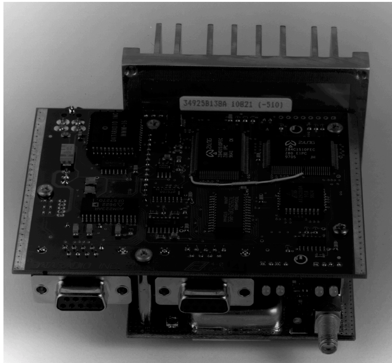
Fig 1. MCUC5 assembly, bottom (loader/modem board) side view
