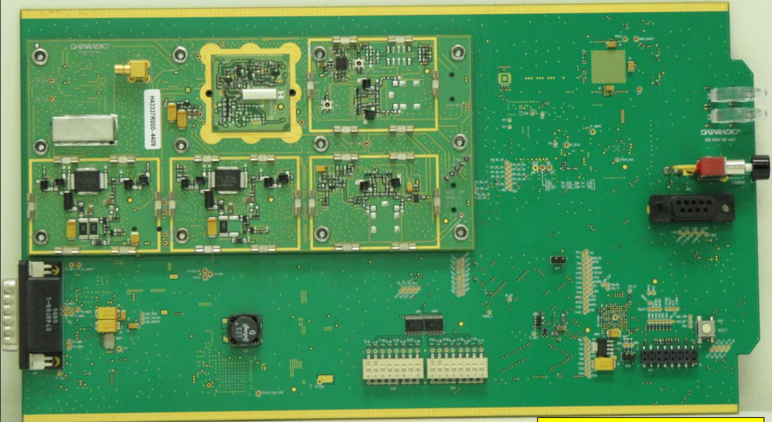
SDR-001-T-403_Internal_Digital-RF-VCO_top_side.pdf
