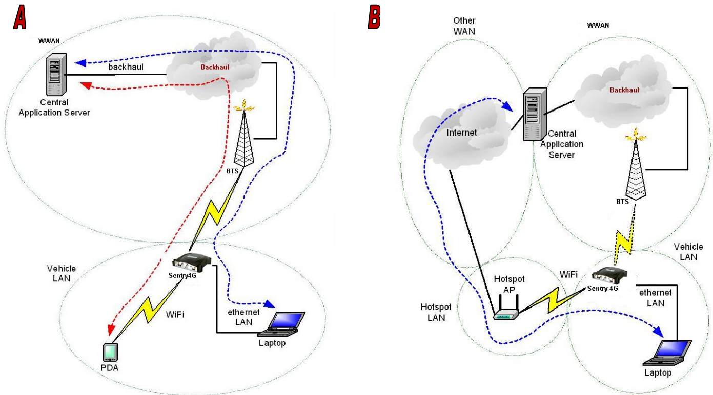
Figure 13 - Sentry 4G WiFi Modes: Access Point (A); Client Mode (B)
