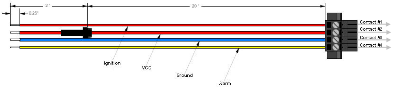
Figure 2 - Dataradio Sentry 4G Power Cable Connections
