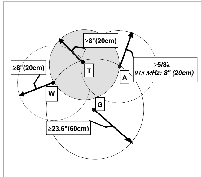
Figure 3 - Antenna Spacing 1
