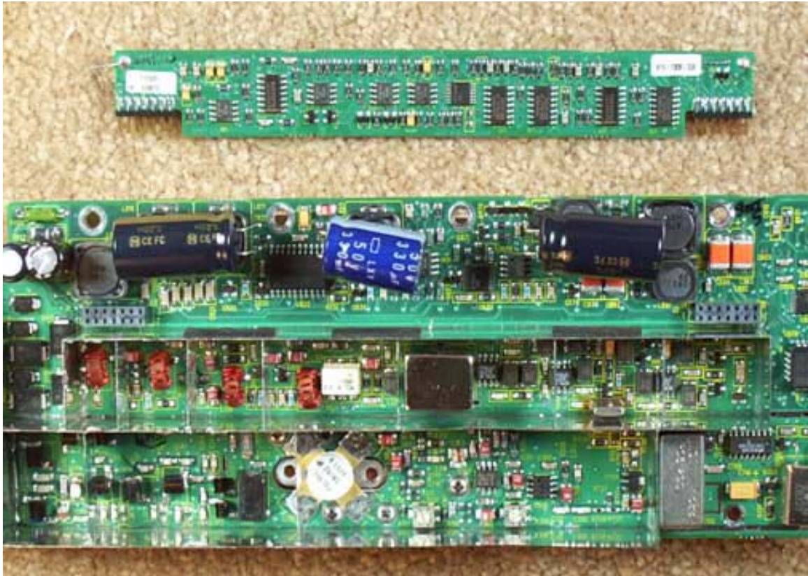
Main PCB Top Audio PCB Location
