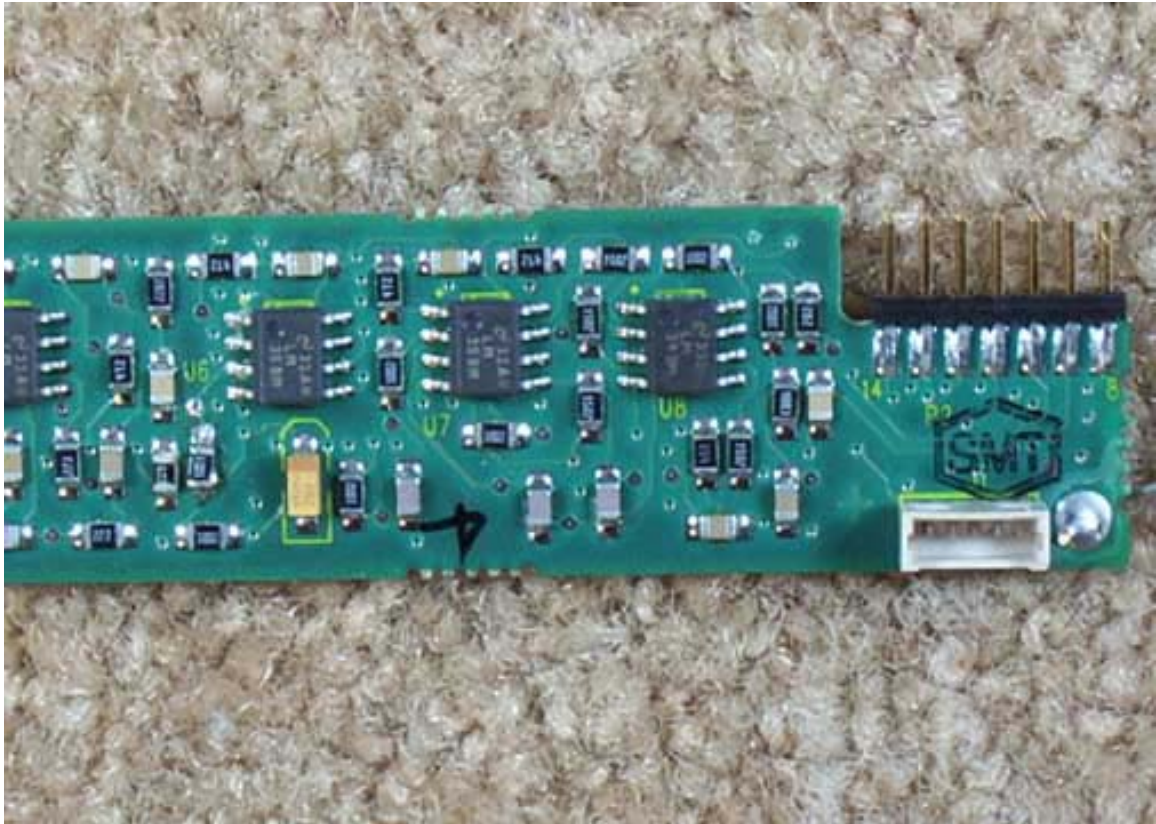
Audio PCB Back Closeup 3
