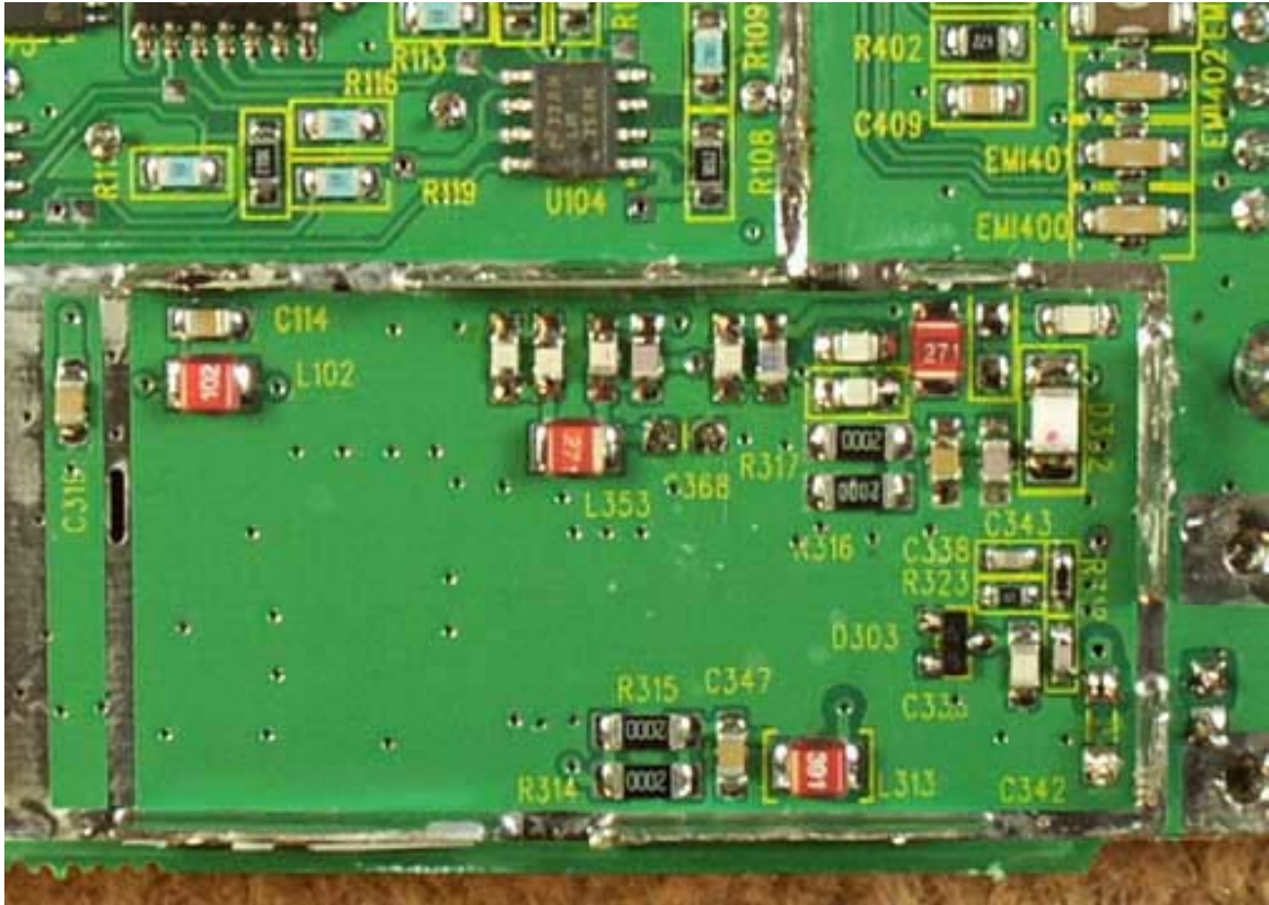
Main PCB Bottom Closeup 7 Shield Removed
