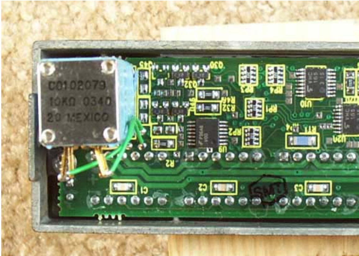
Display PCB Back Closeup 1
