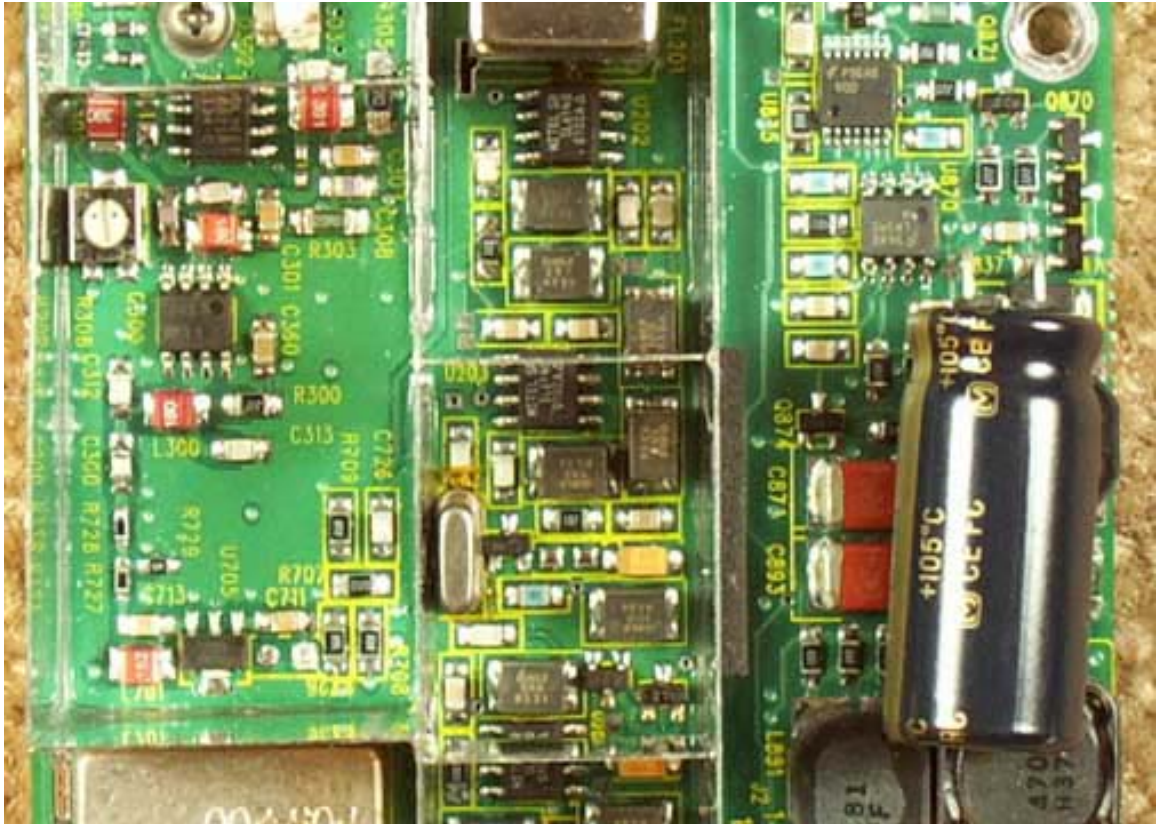
Main PCB Top Closeup 3
