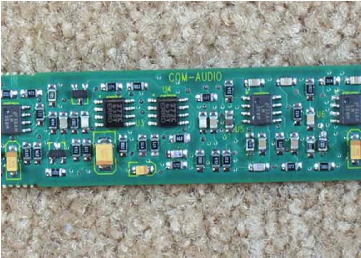
Audio PCB Back Closeup 2
