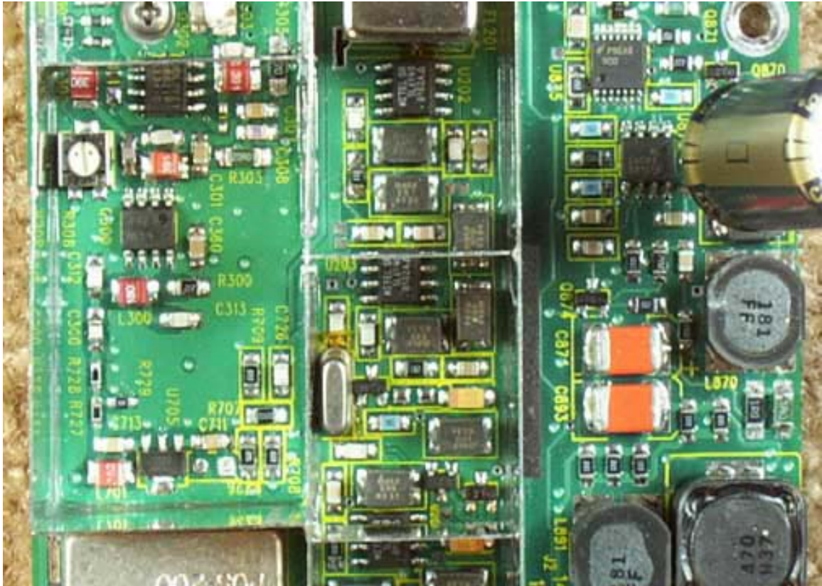
Main PCB Top Closeup 4
