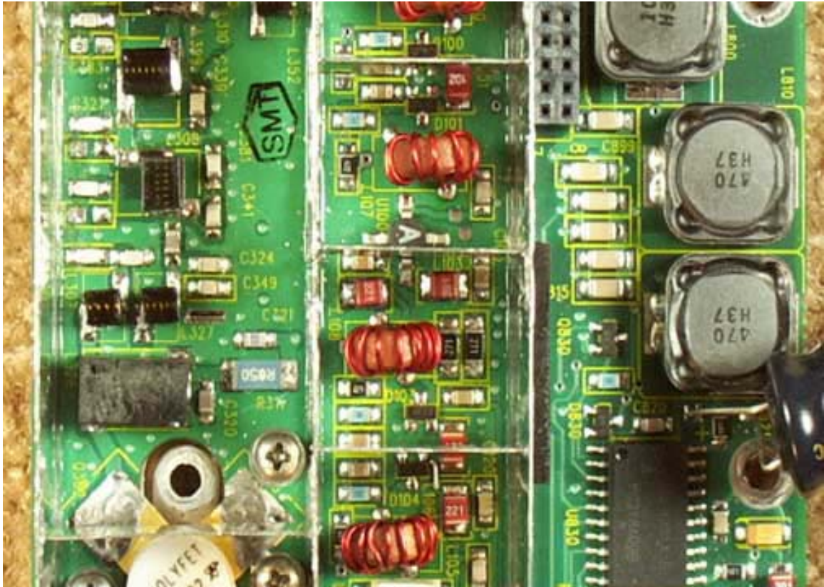
Main PCB Top Closeup 7
