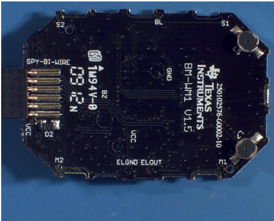
Surflink Watch bottomside internal photo
