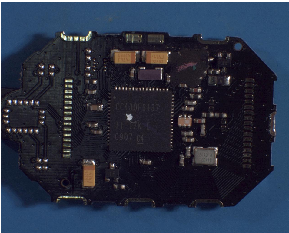
Surflink Watch topside internal photo with display face removed
