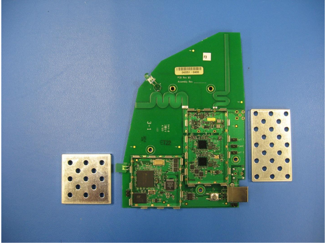
SHARC topside PCB with shields removed
