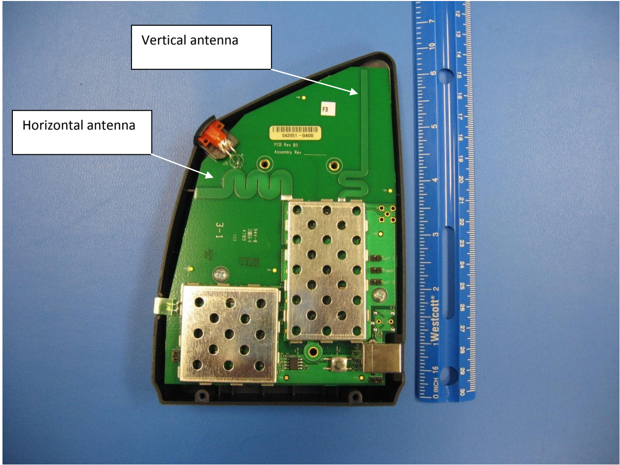
SHARC topside PCB shown mounted in chassis
