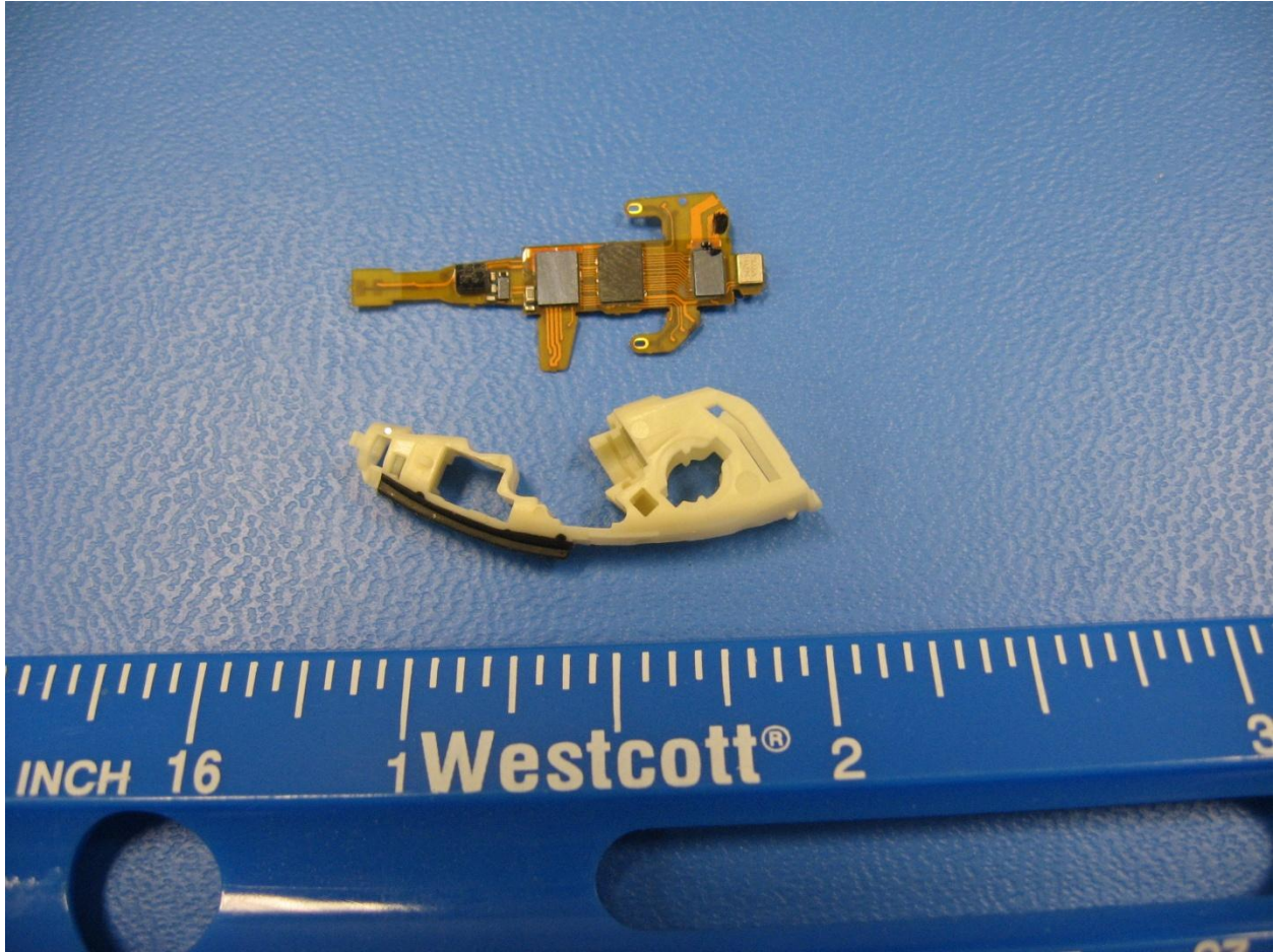
IRIS hearing aid internal construction showing topside flex circuit and mounting frame. Antenna not shown
