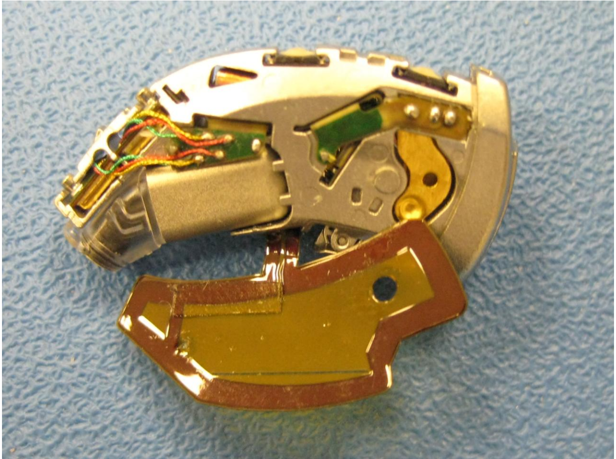
3SERMINI left side with antenna lobe bent down internal photo
