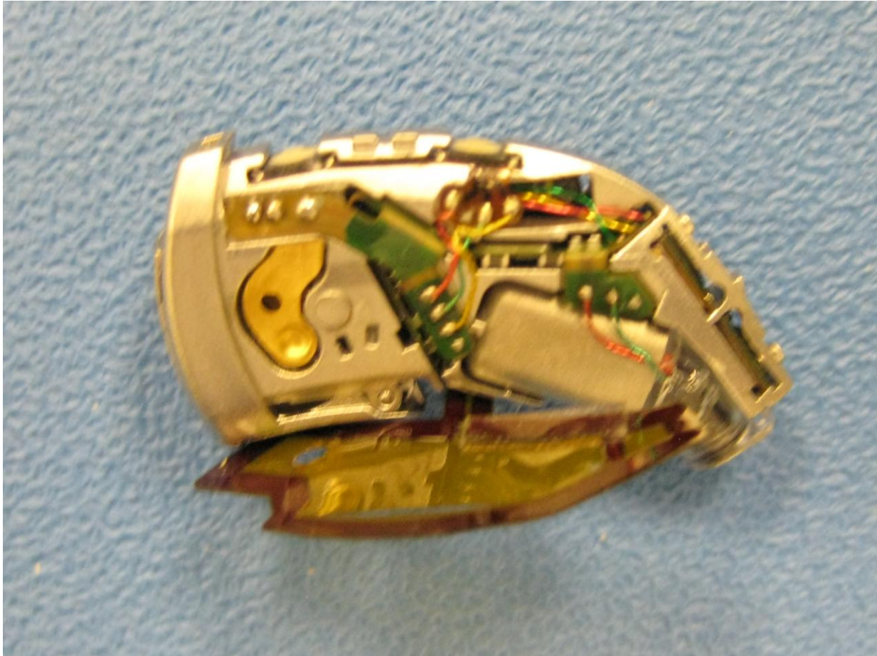
3SERMINI right side with antenna lobe bent down internal photo
