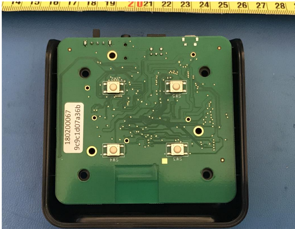
PCB board (top side) in bottom case (scale in cm)
