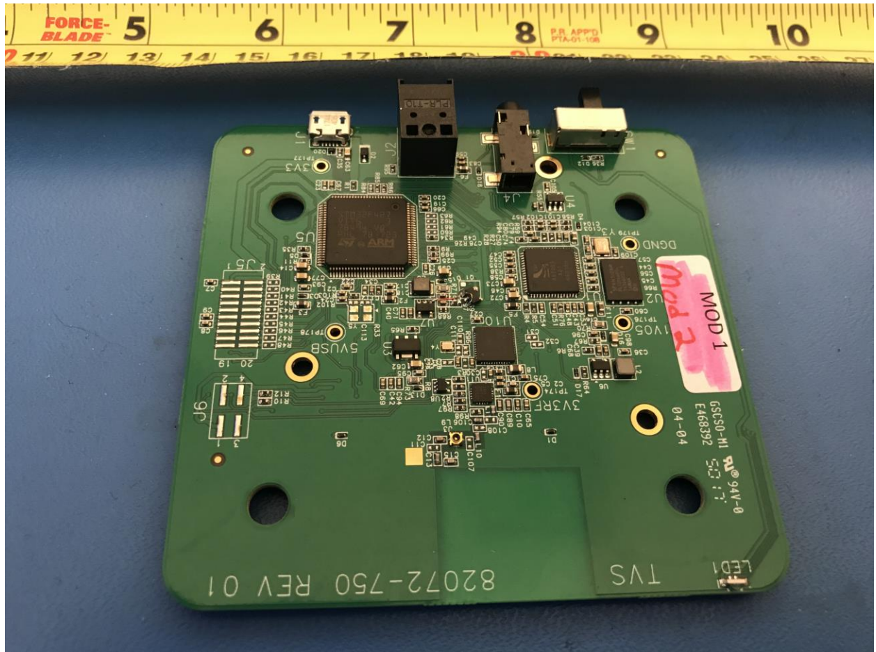
PC board bottom side (scale in inches above scale in cm)
