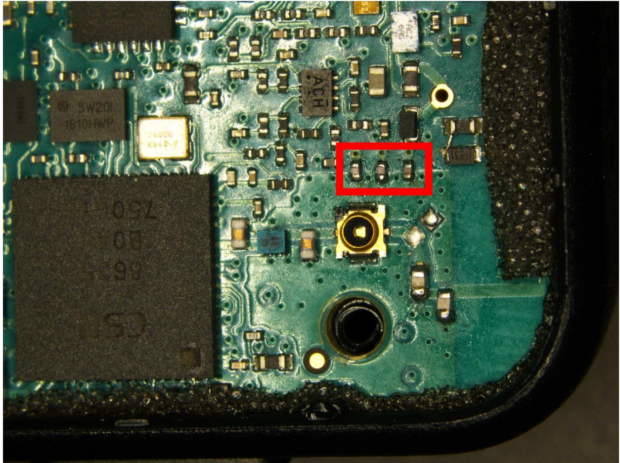
Modified Remote Microphone+ circuit board. Added capacitors shown in red.
