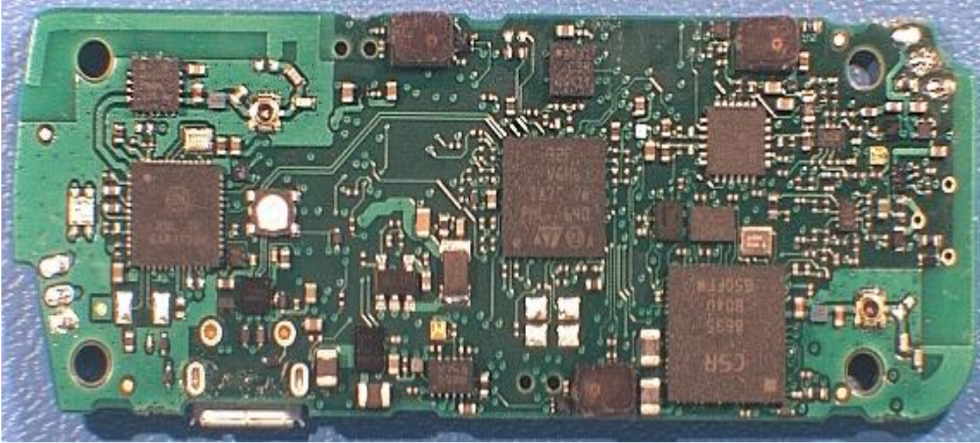
Overall PCB component side, detail views follow
