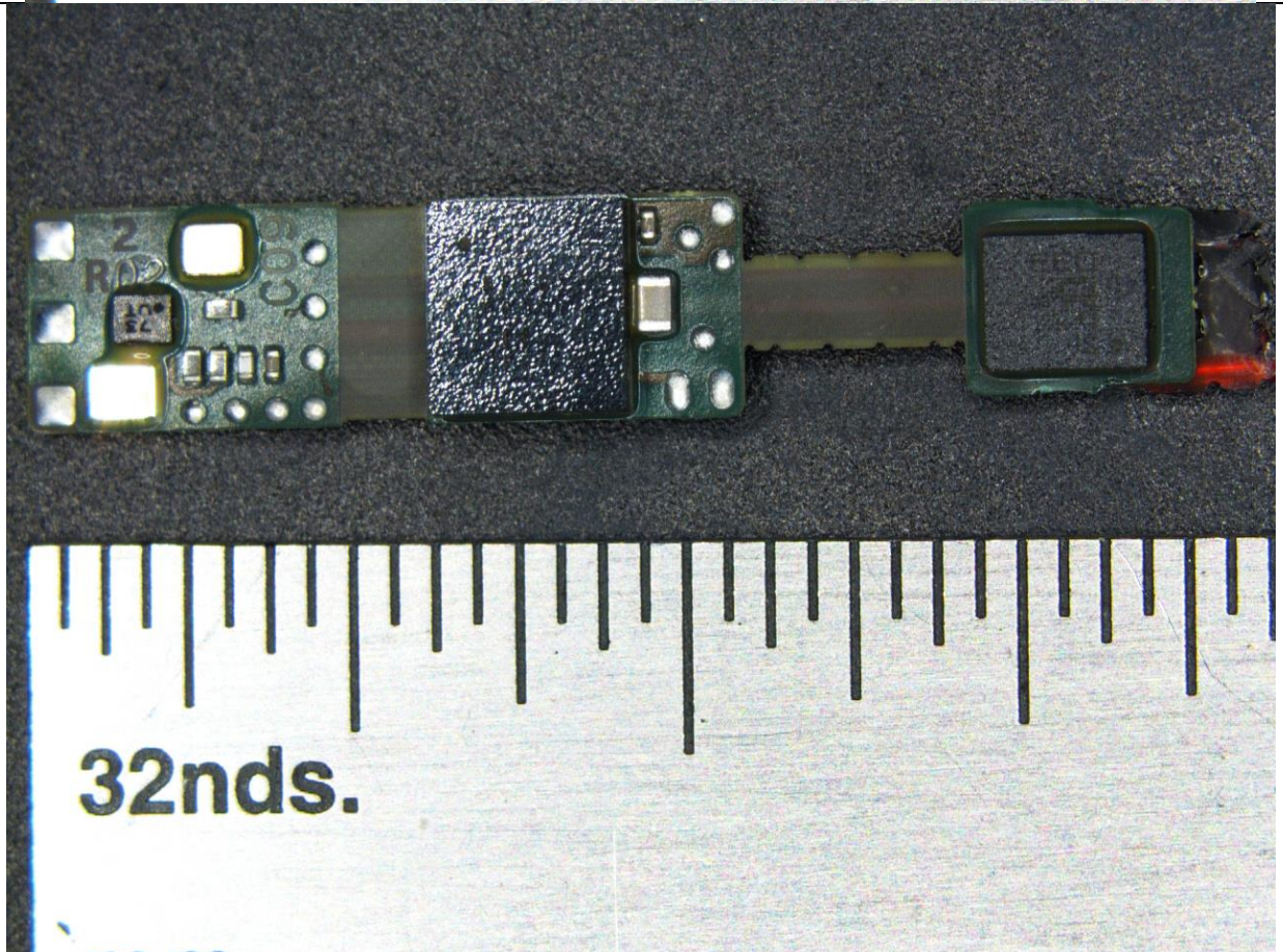
PCB top (scale in inches)
