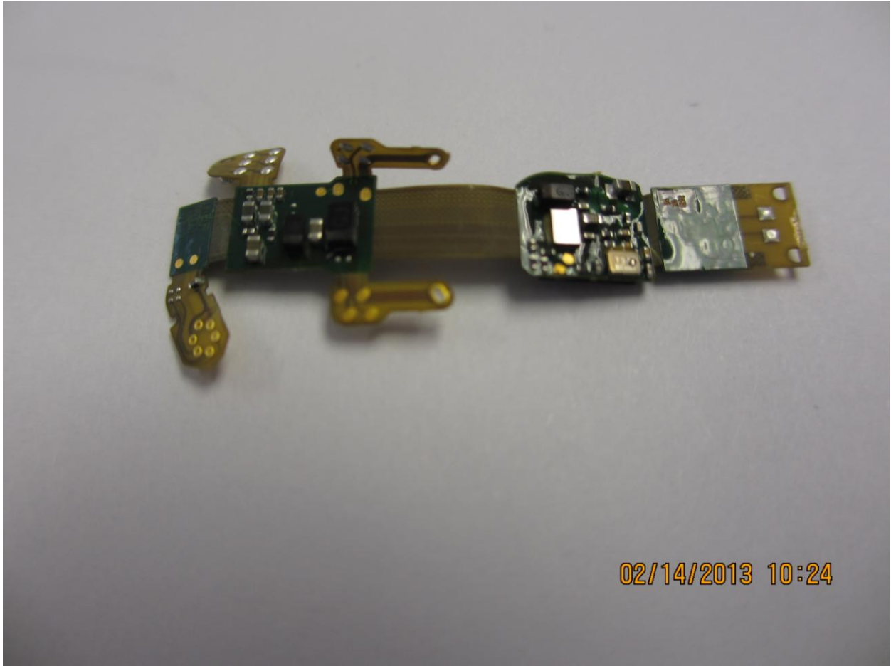
XF13 Internal Photo showing bottomside PCA
