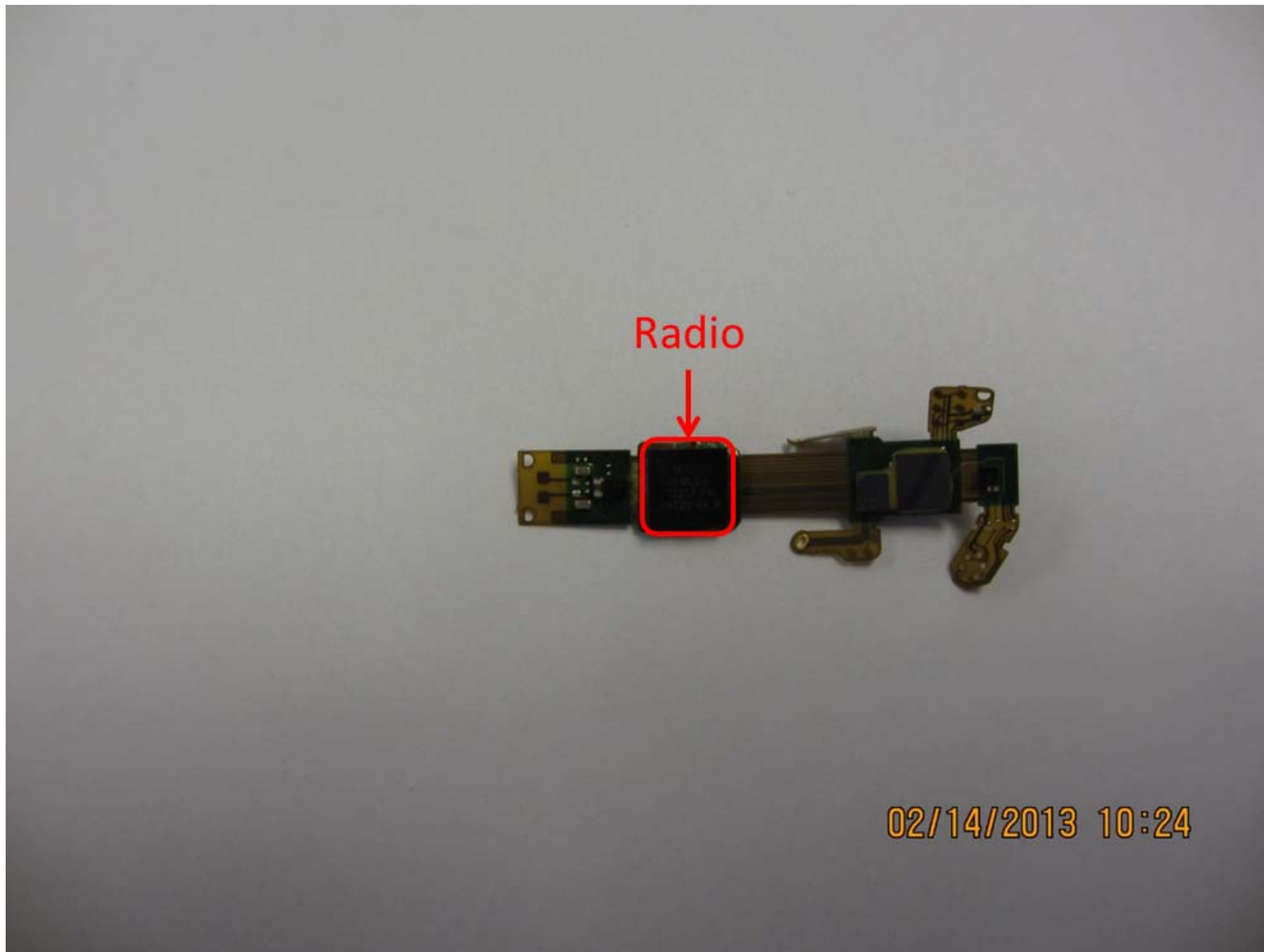
XF13 Internal Photo showing topside PCA
