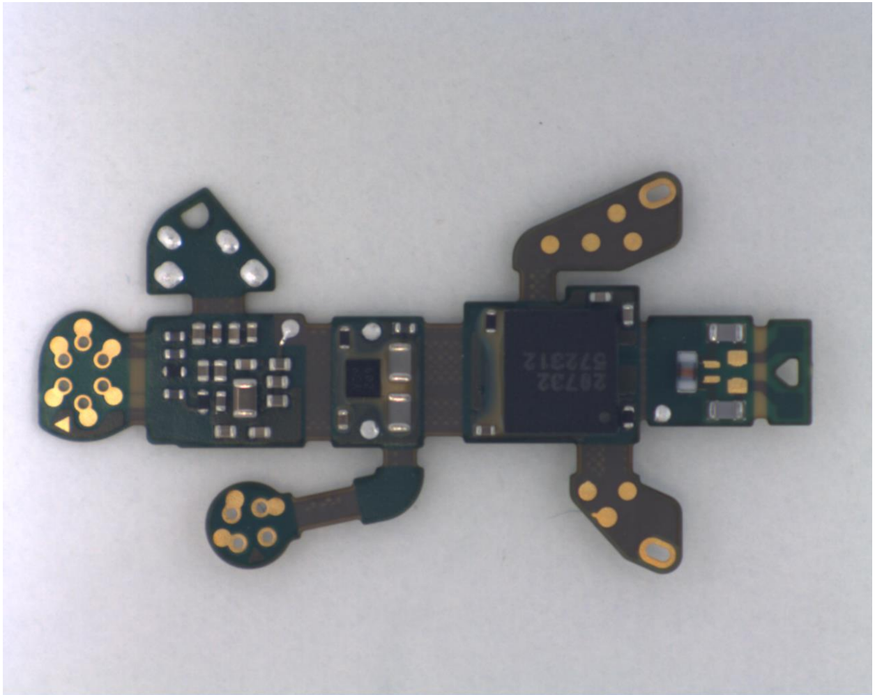
Circuit board front
