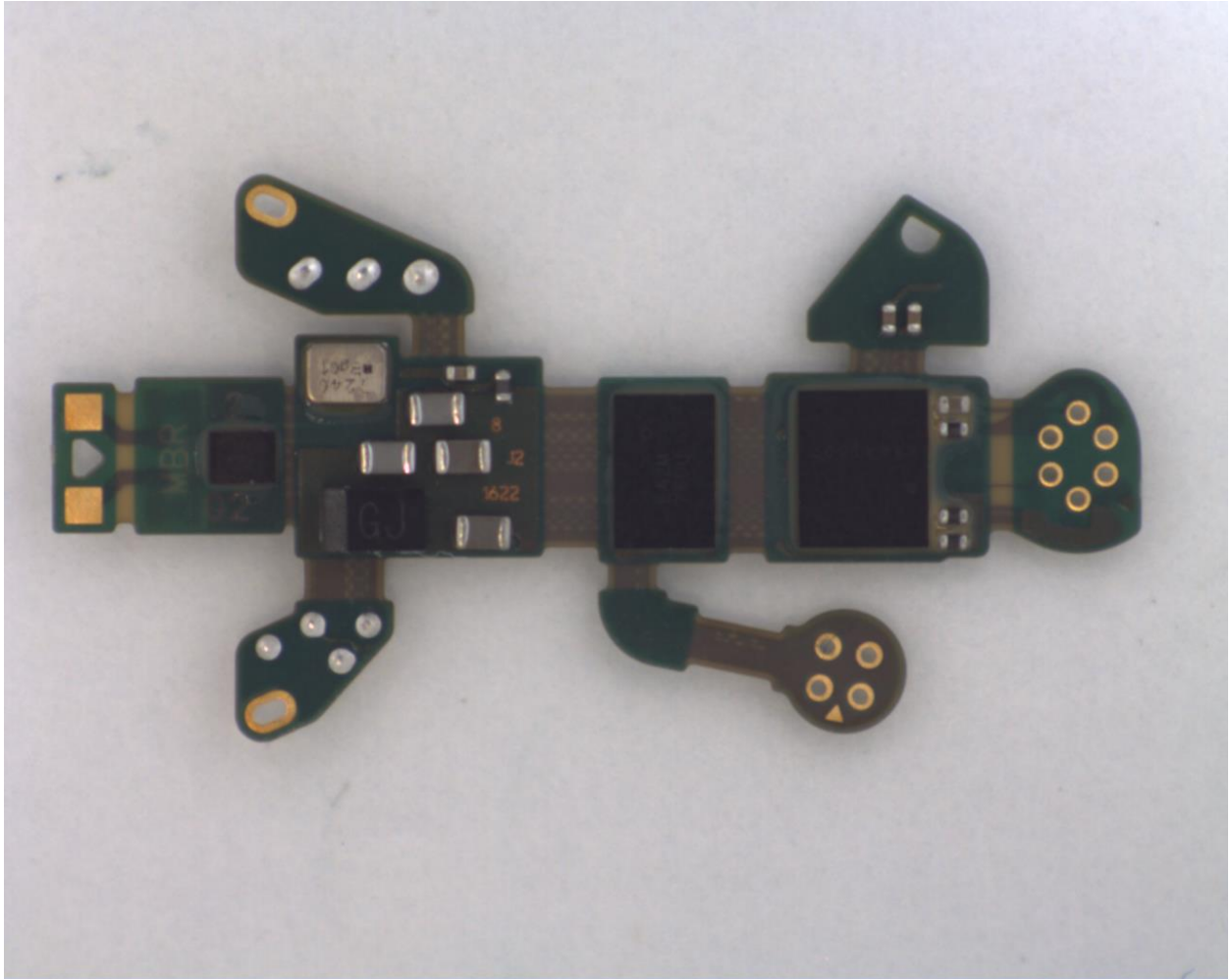
Circuit board back
