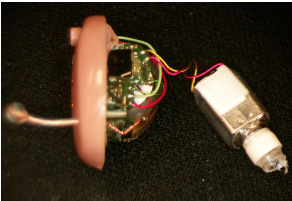
Signature CIC R hearing aid left side view (same for left and right hearing aid)
