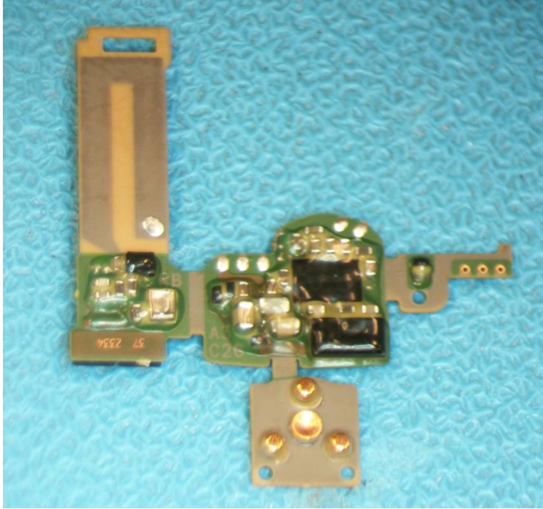
Signature CIC R right hearing aid PCB front side
