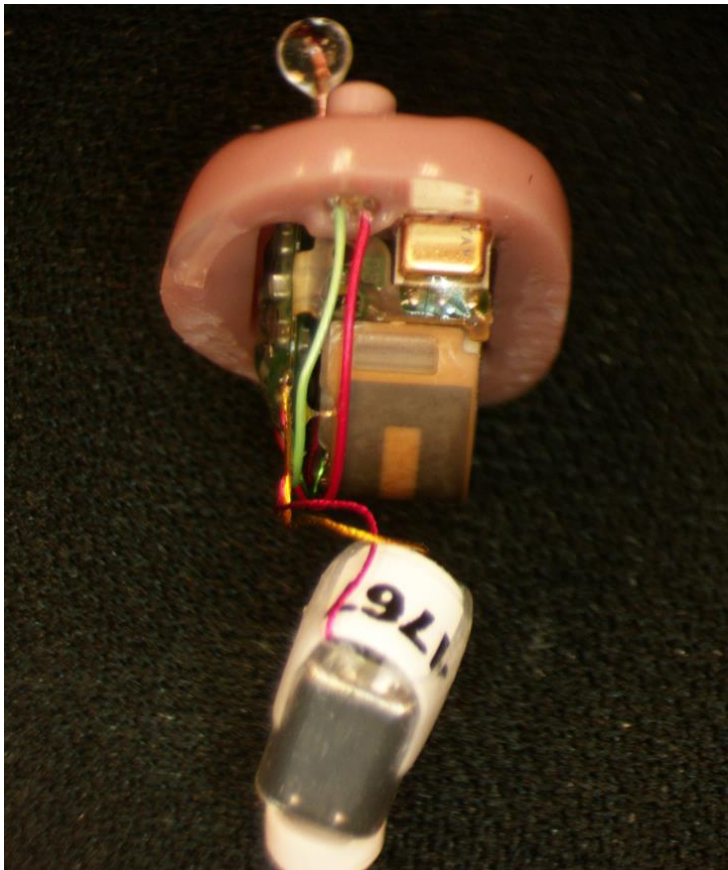
Signature CIC R hearing aid End view 2 (same for left and right hearing aid)
