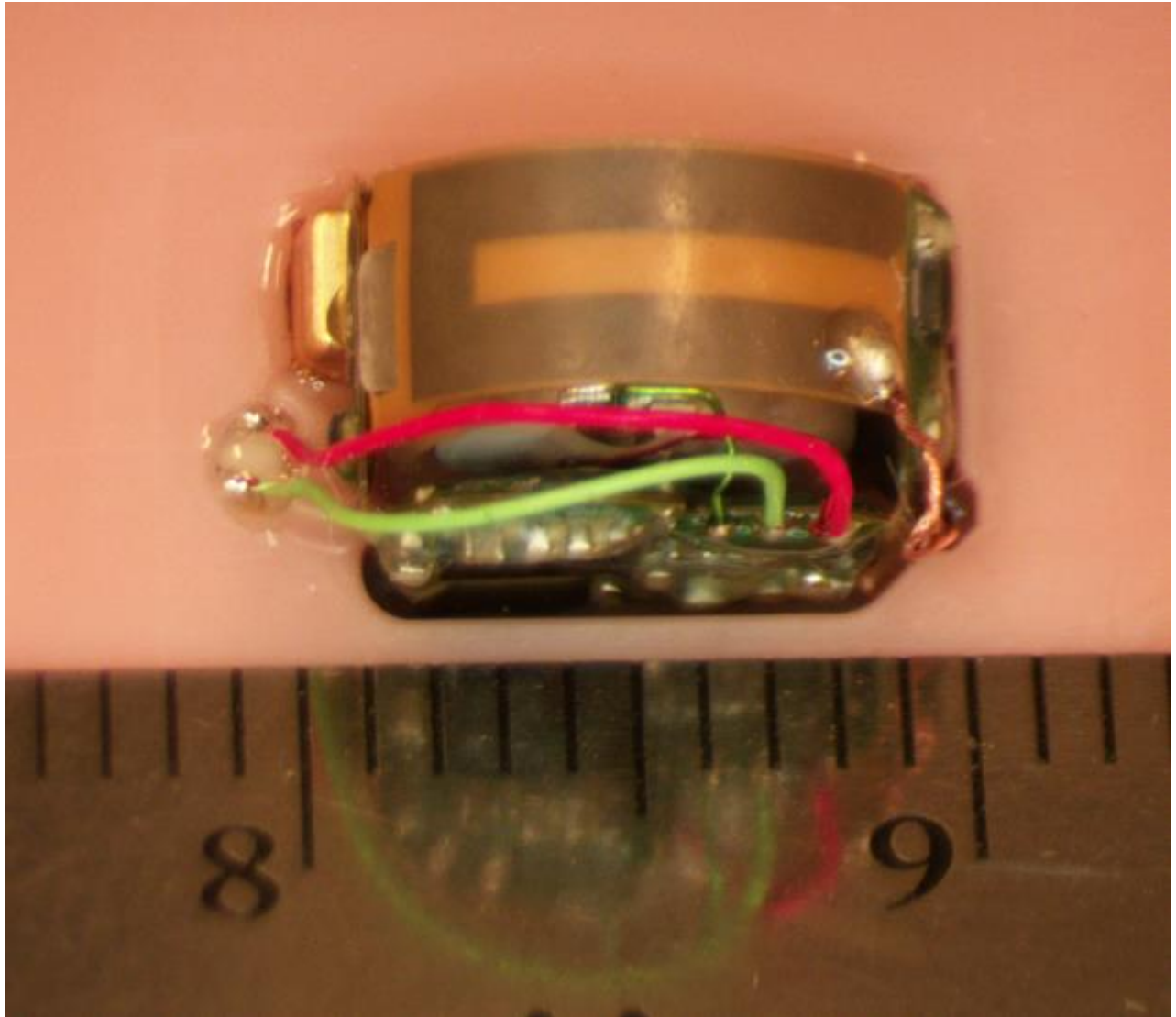
Signature CIC R PCBA front view (same for left and right hearing aid)
