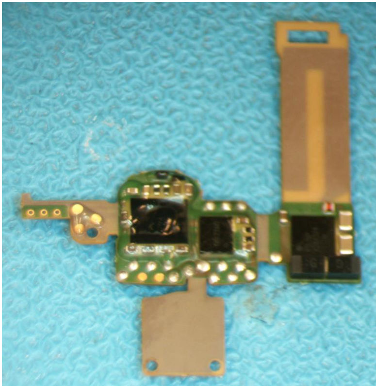
Signature CIC R right hearing aid PCB back side
