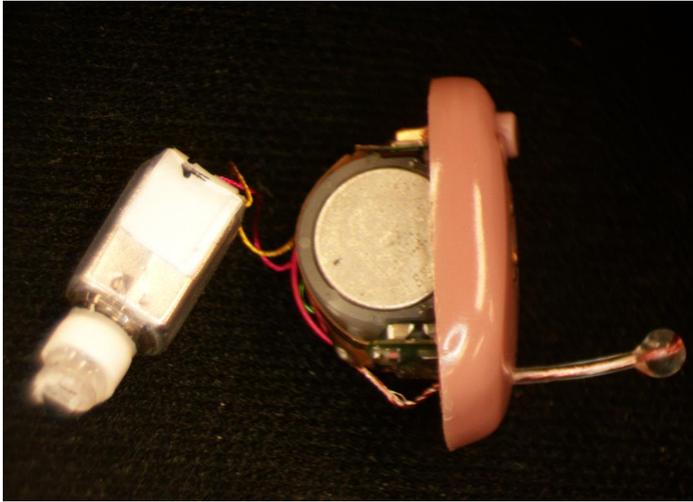
Signature CIC R hearing aid right side view (same for left and right hearing aid)
