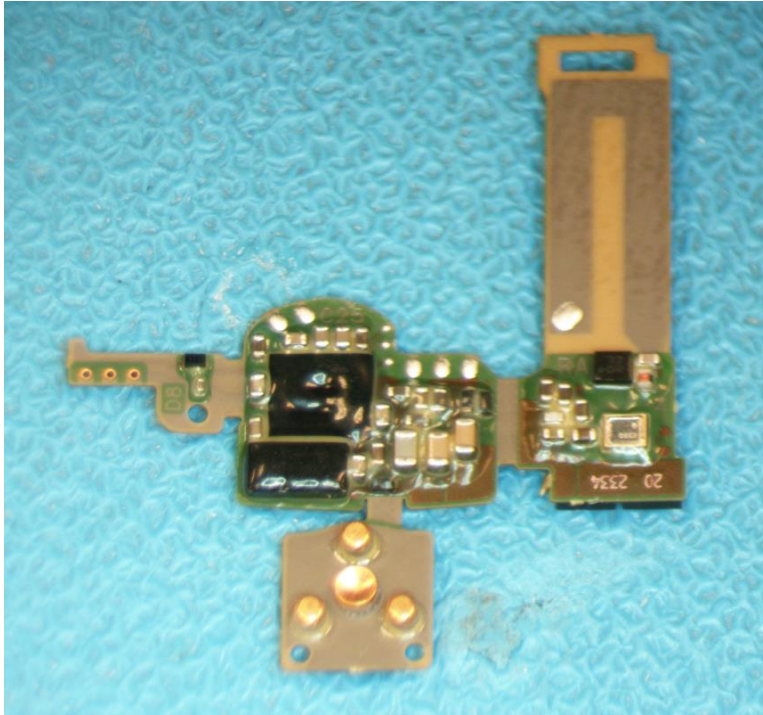
Signature CIC R left hearing aid PCB front side
