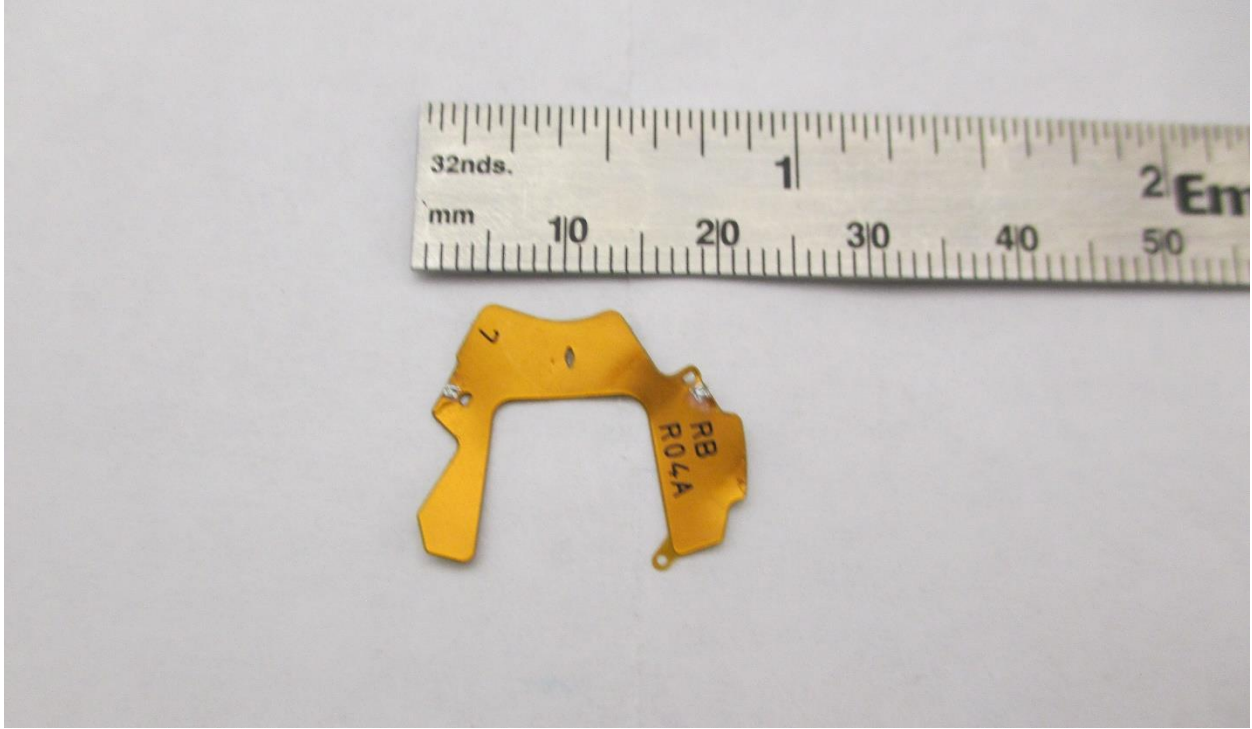
Unfolded antenna
