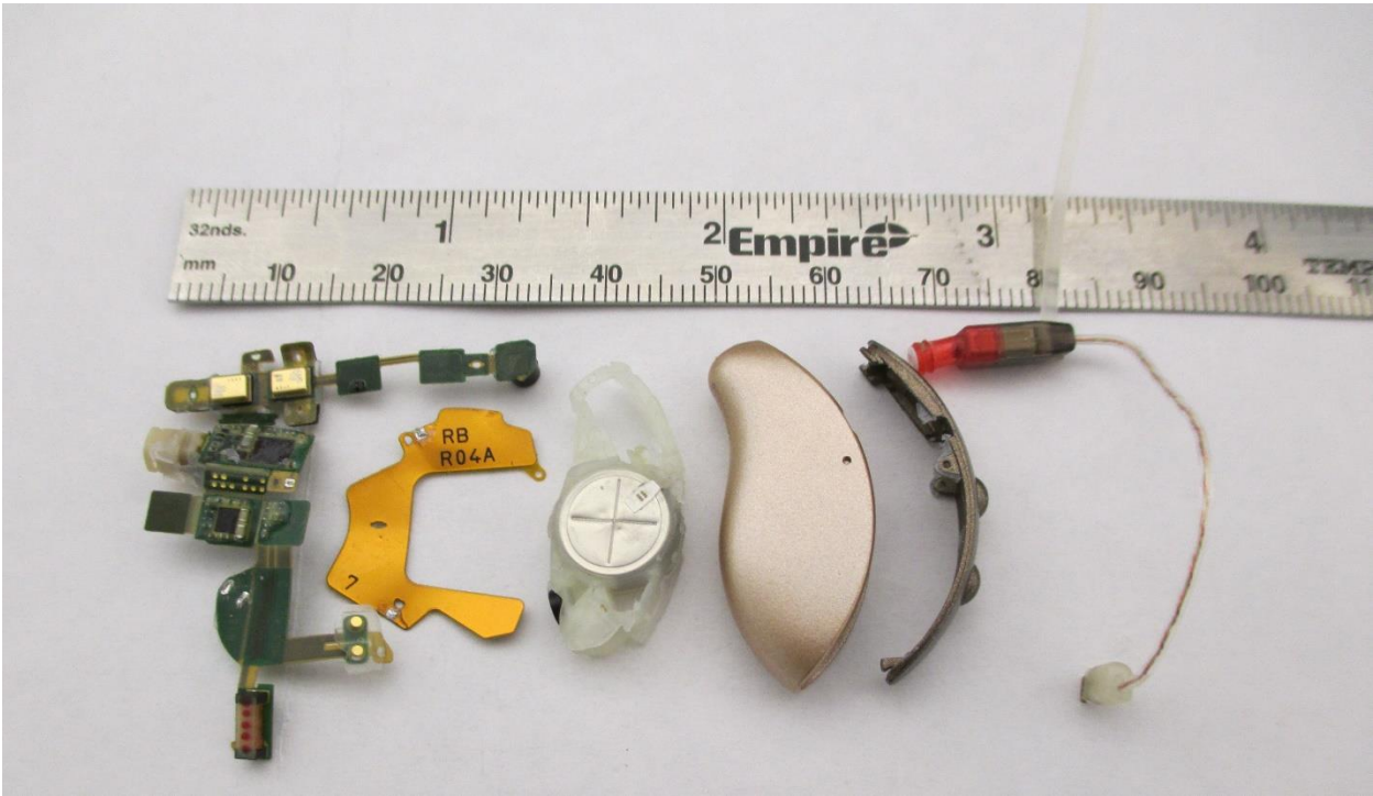
Overall assembly
