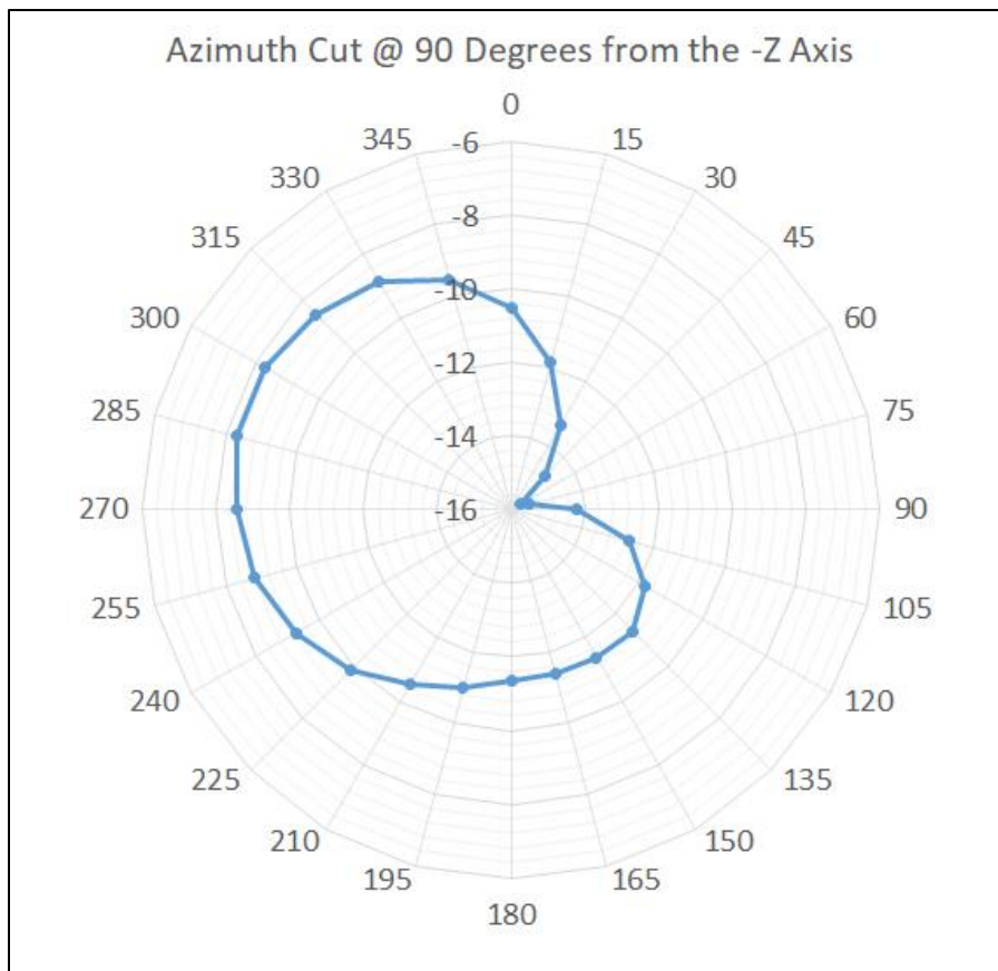
Figure 2b Hearing Aid Antenna Elevation and Azimuth Cuts
