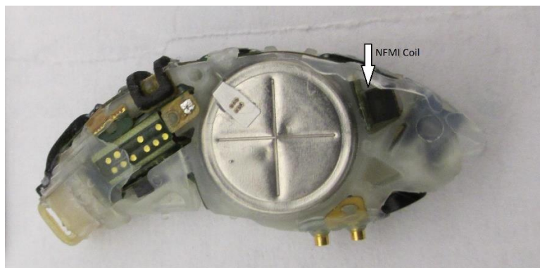
Figure 4c NFMI Antenna in Assembled Hearing Aid
