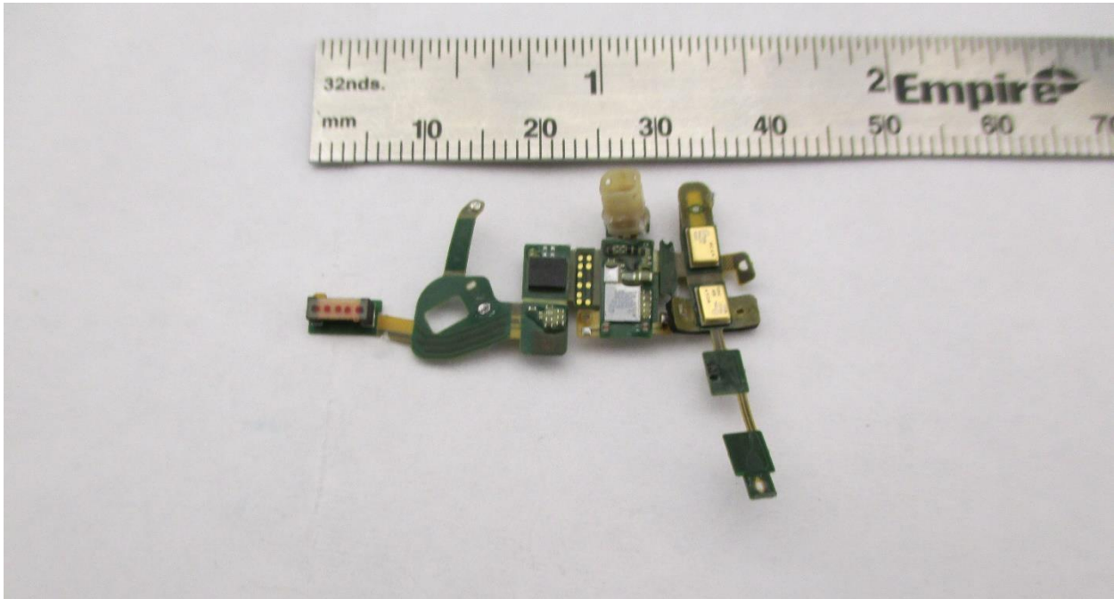
PCBA front
