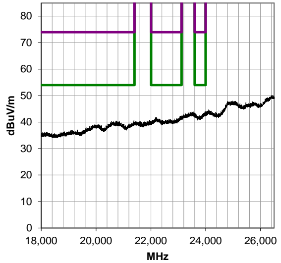
18000-26500 MHz, Run 32
