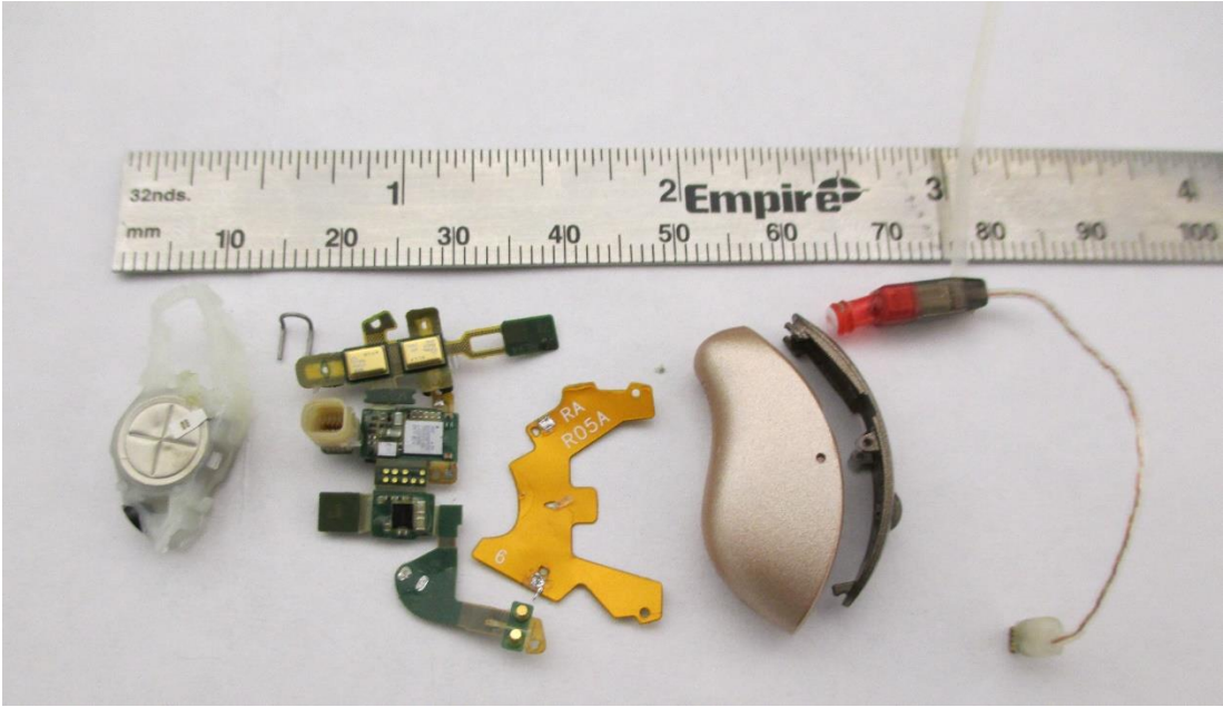
Overall assembly
