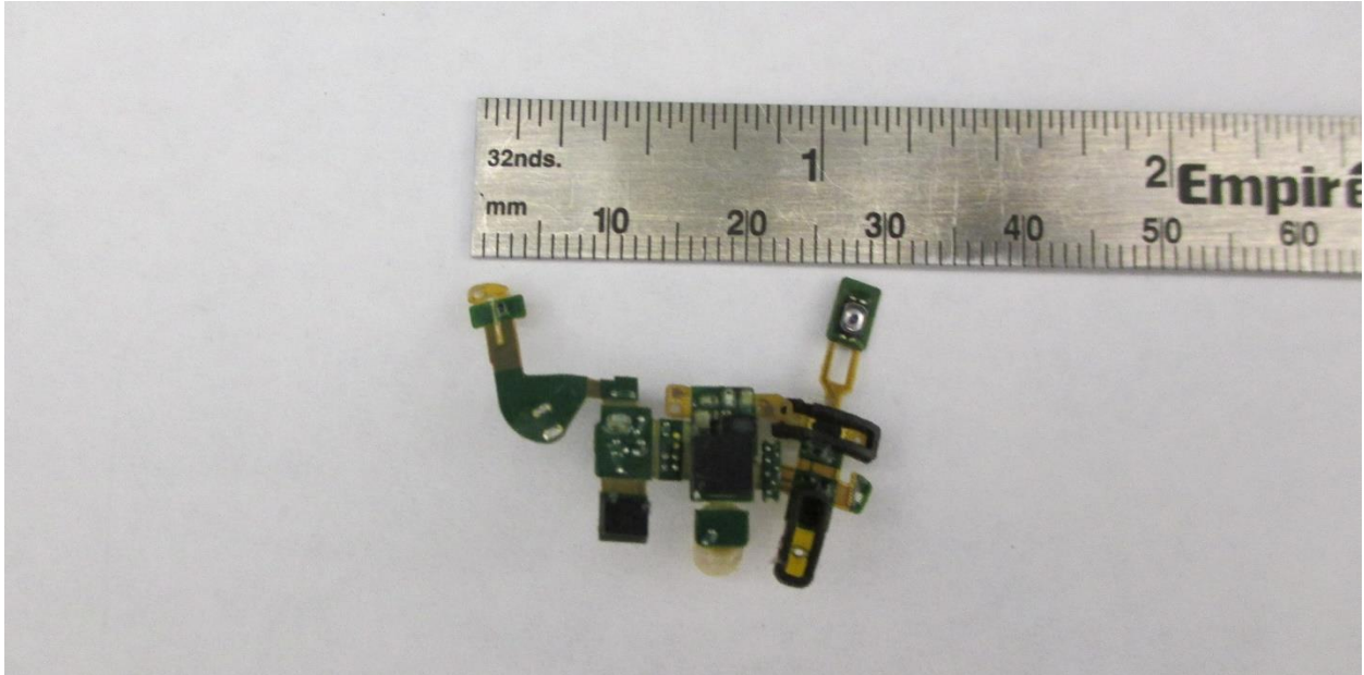
PCBA back
