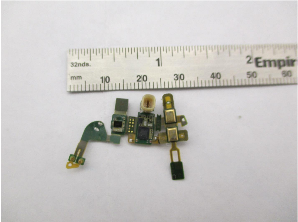
PCBA front
