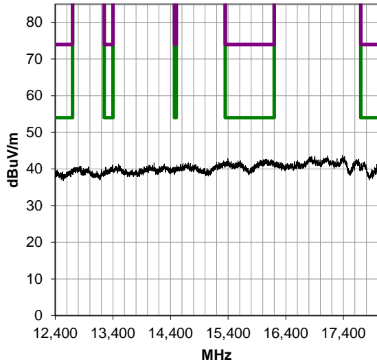
12400-18000 MHz, Run 22
