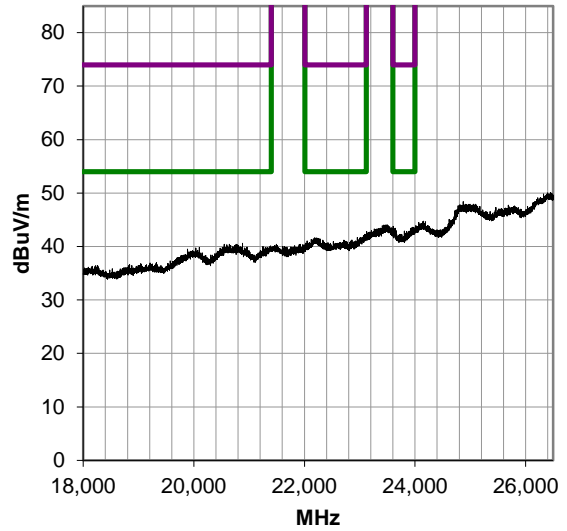
18000-26500 MHz, Run 34
