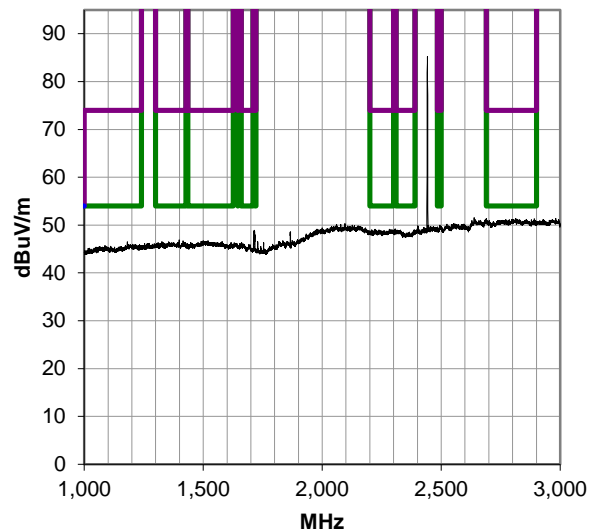
1000-3000 MHz, Run 19
