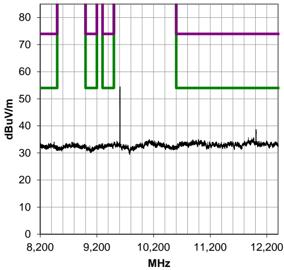
8200-12400 MHz, Run 4
