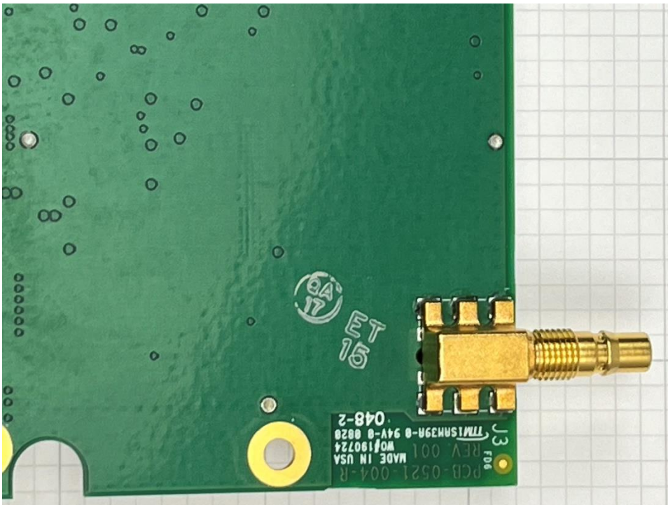
2.11 PCA-0521-204-R (CAM3 RF, CISCO IR8140) Back, Detail 2
