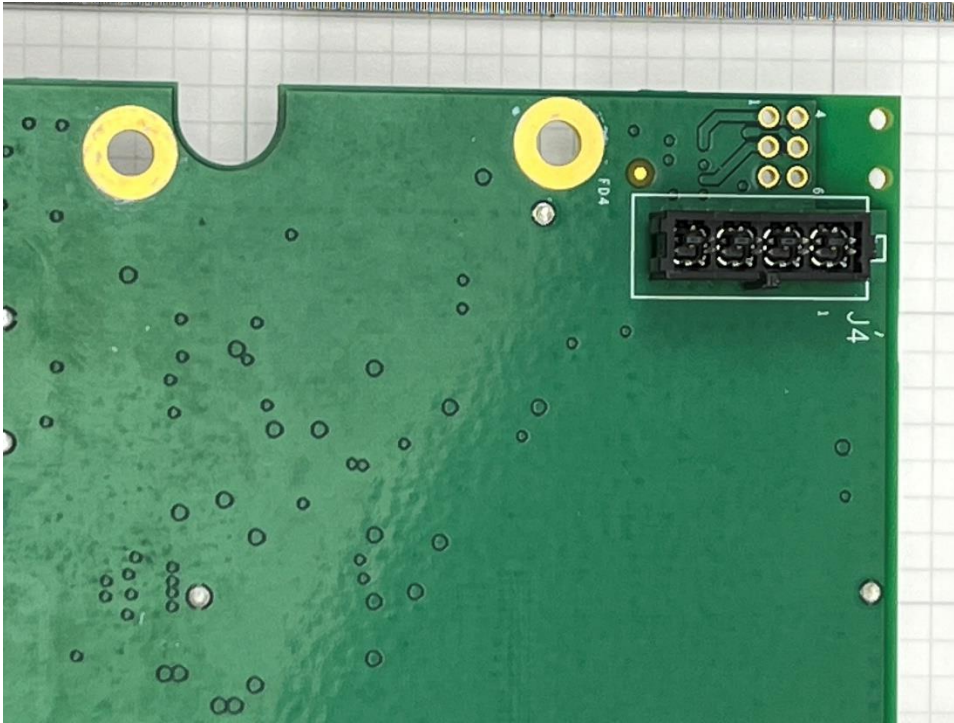
2.10 PCA-0521-204-R (CAM3 RF, CISCO IR8140) Back, Detail 1
