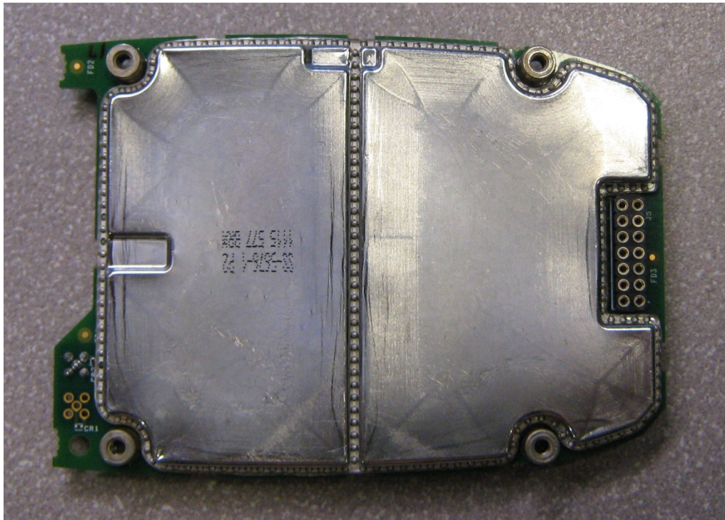
RF Module with shield, Bottom
